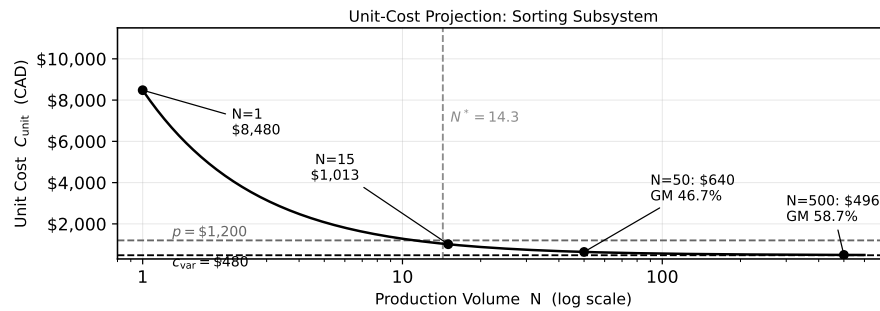
Figure 17.2: C_{\text{unit}}(N) for the IoT sorting subsystem on a log N -axis. The curve falls from $8,480 at N = 1 to $496 at N = 500 , asymptoting to c_{\text{var}} = \$480 (lower dashed line). The selling price p = \$1,200 is marked by the upper dashed line; the vertical dashed line at N^* = 14.3 is the process break-even from Chapter 12. Annotated arrows show gross margin at N = 50 (46.7%) and N = 500 (58.7%).
