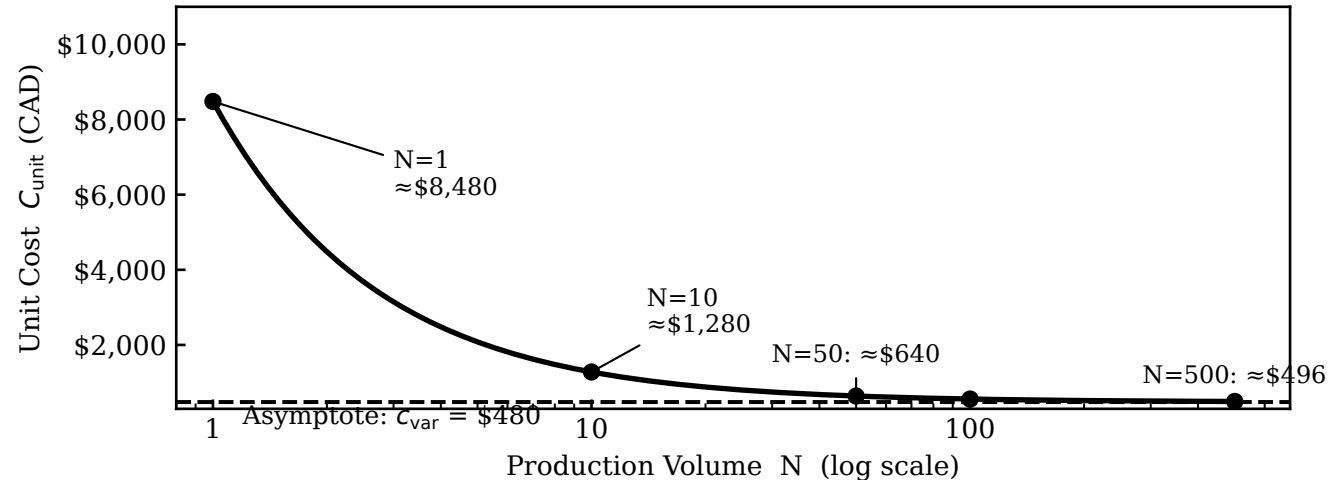
Unit Cost vs. Production Volume
