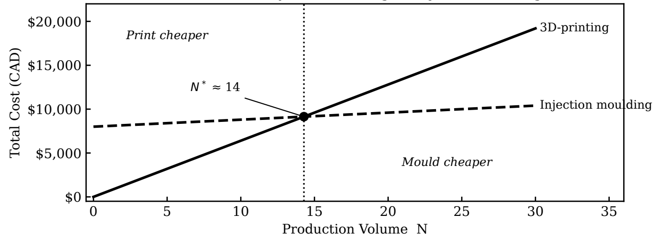
Break-Even Analysis: 3D-Printing vs. Injection Moulding
