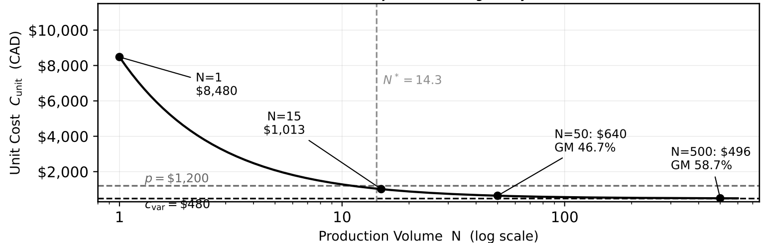
Unit-Cost Projection: Sorting Subsystem
