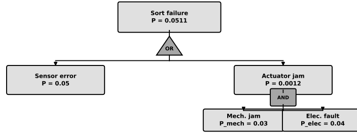
Figure 14.4: Two-level fault tree for the sorting subsystem. The OR gate at top combines “Sensor error” (dominant path) and “Actuator jam” (AND of mechanical and electrical faults). P(\text{top}) \approx 5.11\% .
