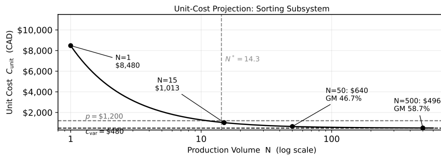
Figure 17.2: C_{\text{unit}}(N) for the IoT sorting subsystem on a log N -axis. The curve falls from $8,480 at N = 1 to $496 at N = 500 , asymptotically to c_{\text{var}} = \$480 (lower dashed line). The selling price p = \$1,200 is marked by the upper dashed line; the vertical dashed line at N^* = 14.3 is the process break-even from Chapter 12. Annotated arrows show gross margin at N = 50 (46.7%) and N = 500 (58.7%).
