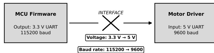
Figure 5.3: Boundary mismatch at integration. The left subsystem (MCU firmware) assumes 3.3 V CMOS logic and outputs a valid signal by its own standard; the right subsystem (motor driver) expects 5 V TTL and interprets the same signal as an indeterminate logic level. Neither subsystem contains a bug in isolation; the defect exists only at the boundary, and is invisible until the two are connected.
