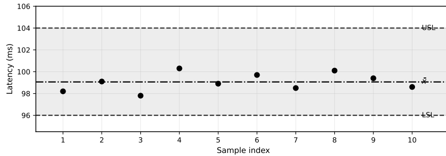
Figure 14.2: Ten latency measurements plotted against the LSL–USL tolerance band. All measurements fall comfortably within the specification.
