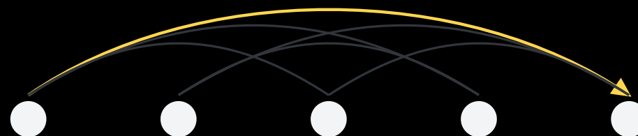
Self-attention
