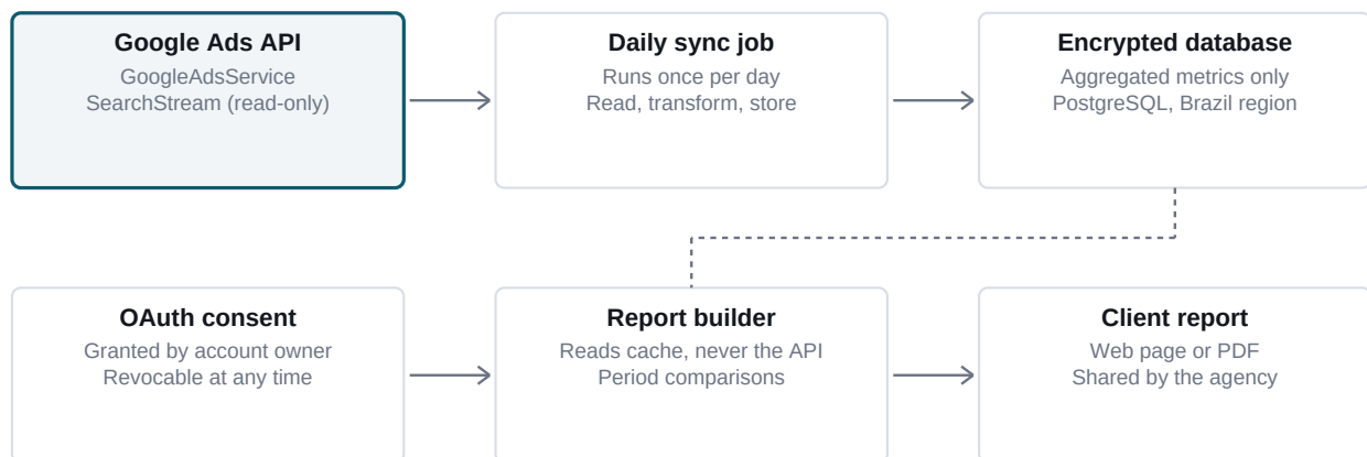
Figure 1 - Data flow from OAuth consent to the delivered report.
