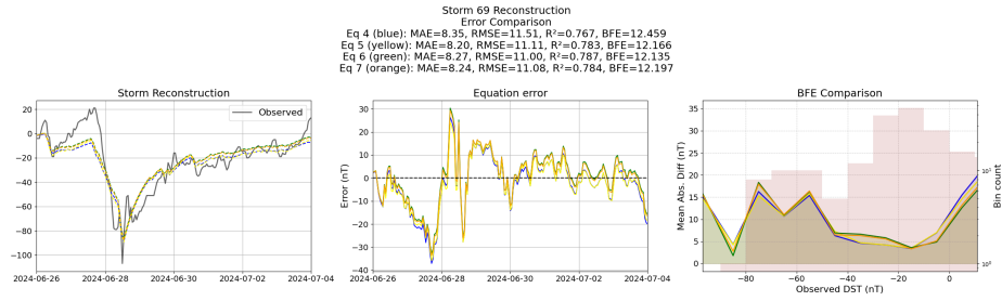
Figure 36: Reconstruction of storm 69 using the Equations generated from the unconstrained symbolic regression with the derived features
