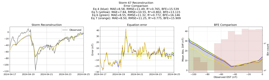
Figure 34: Reconstruction of storm 67 using the Equations generated from the unconstrained symbolic regression with the derived features
