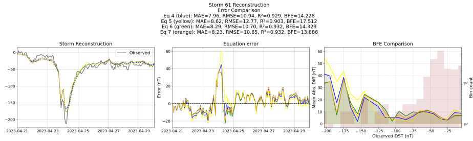
Figure 28: Reconstruction of storm 61 using the Equations generated from the unconstrained symbolic regression with the derived features
