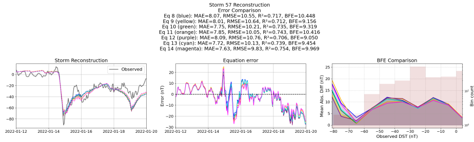
Figure 44: Reconstruction of storm 57 using the Equations generated from the templated symbolic regression with the primitive features
