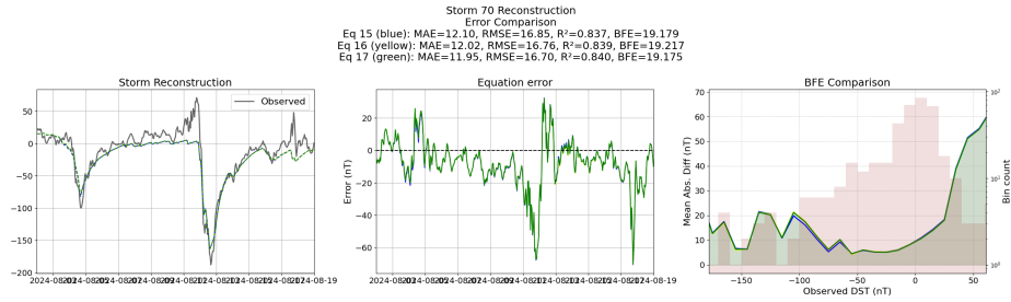
Figure 77: Reconstruction of storm 70 using the Equations generated from the templated symbolic regression with the derived features
