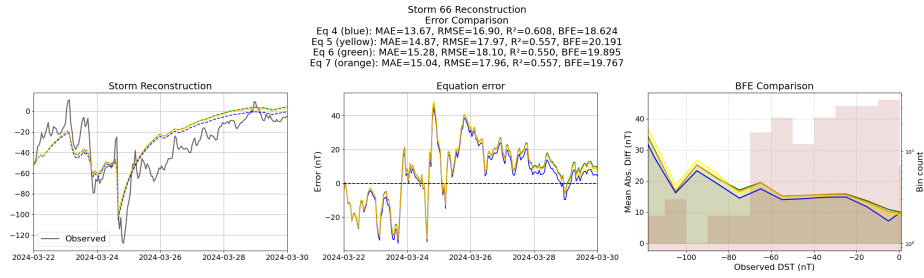
Figure 33: Reconstruction of storm 66 using the Equations generated from the unconstrained symbolic regression with the derived features
