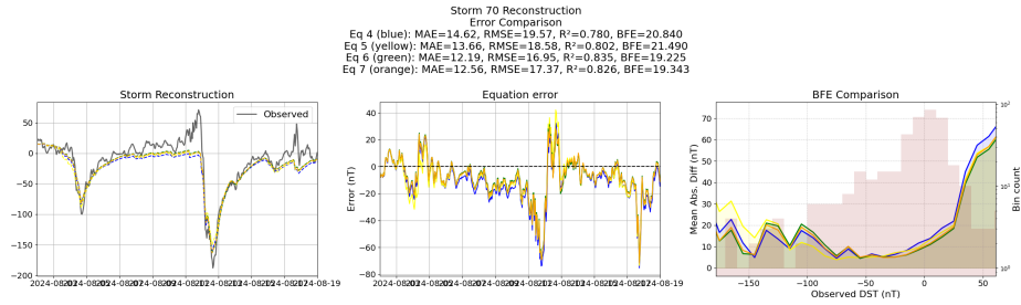
Figure 37: Reconstruction of storm 70 using the Equations generated from the unconstrained symbolic regression with the derived features
