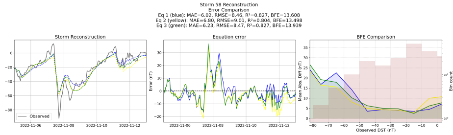
Figure 5: Reconstruction of storm 58 using the Equations generated from the unconstrained symbolic regression with the primitive features
