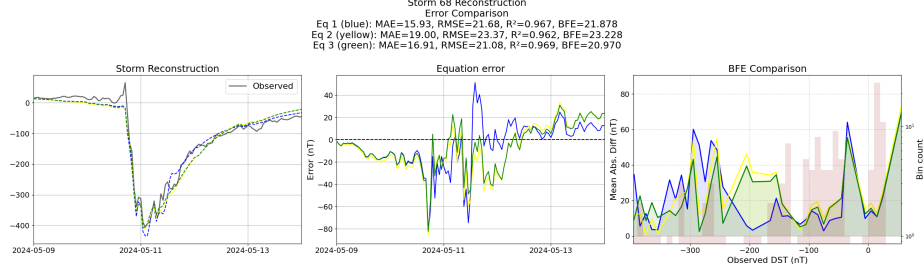
Figure 15: Reconstruction of storm 68 using the Equations generated from the unconstrained symbolic regression with the primitive features
