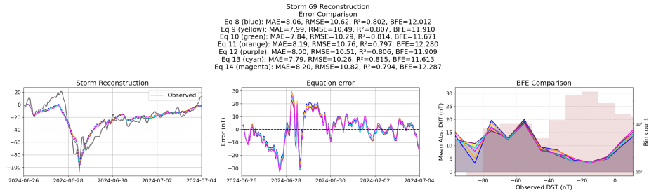
Figure 56: Reconstruction of storm 69 using the Equations generated from the templated symbolic regression with the primitive features
