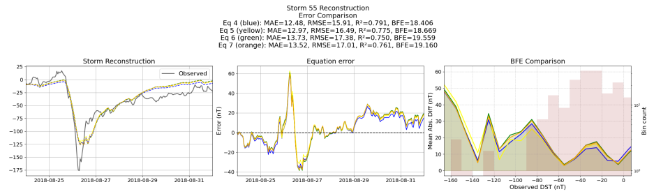
Figure 22: Reconstruction of storm 55 using the Equations generated from the unconstrained symbolic regression with the derived features
