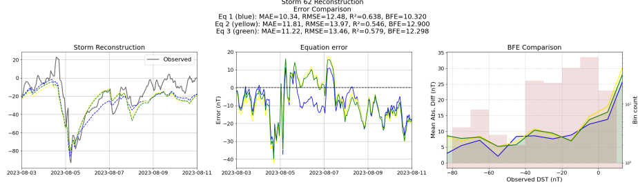
Figure 9: Reconstruction of storm 62 using the Equations generated from the unconstrained symbolic regression with the primitive features
