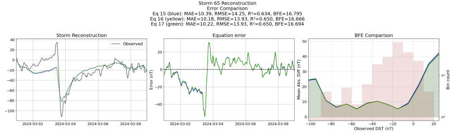
Figure 72: Reconstruction of storm 65 using the Equations generated from the templated symbolic regression with the derived features
