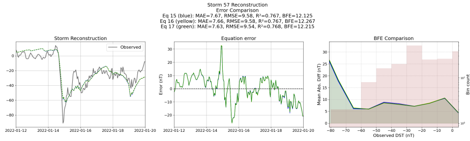
Figure 64: Reconstruction of storm 57 using the Equations generated from the templated symbolic regression with the derived features
