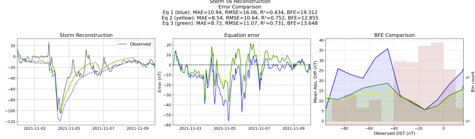
Figure 3: Reconstruction of storm 56 using the Equations generated from the unconstrained symbolic regression with the primitive features
