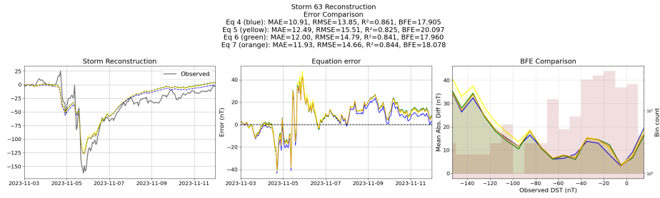
Figure 30: Reconstruction of storm 63 using the Equations generated from the unconstrained symbolic regression with the derived features
