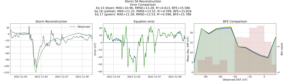
Figure 63: Reconstruction of storm 56 using the Equations generated from the templated symbolic regression with the derived features
