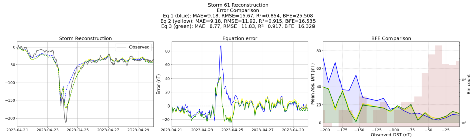
Figure 8: Reconstruction of storm 61 using the Equations generated from the unconstrained symbolic regression with the primitive features
