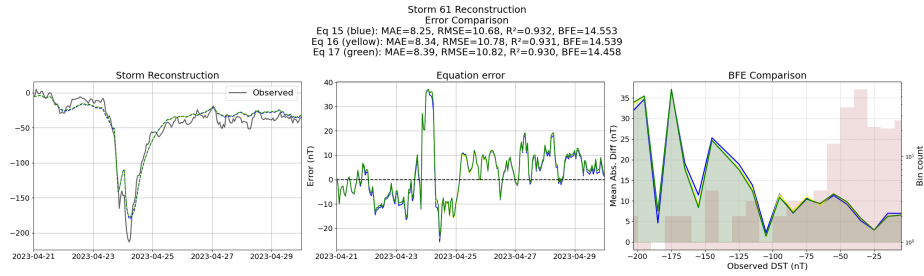
Figure 68: Reconstruction of storm 61 using the Equations generated from the templated symbolic regression with the derived features
