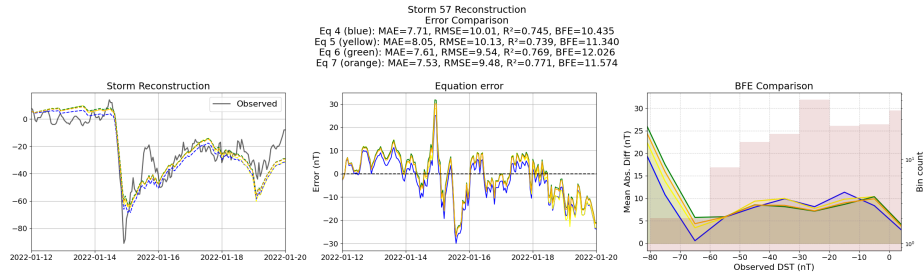
Figure 24: Reconstruction of storm 57 using the Equations generated from the unconstrained symbolic regression with the derived features
