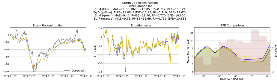
Figure 40: Reconstruction of storm 73 using the Equations generated from the unconstrained symbolic regression with the derived features
