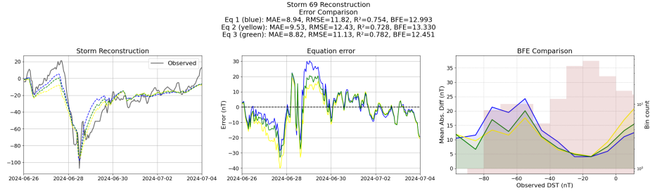
Figure 16: Reconstruction of storm 69 using the Equations generated from the unconstrained symbolic regression with the primitive features
