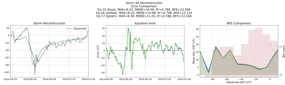
Figure 76: Reconstruction of storm 69 using the Equations generated from the templated symbolic regression with the derived features
