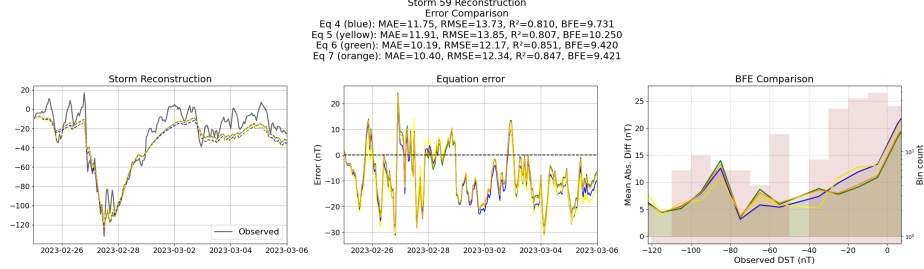
Figure 26: Reconstruction of storm 59 using the Equations generated from the unconstrained symbolic regression with the derived features
