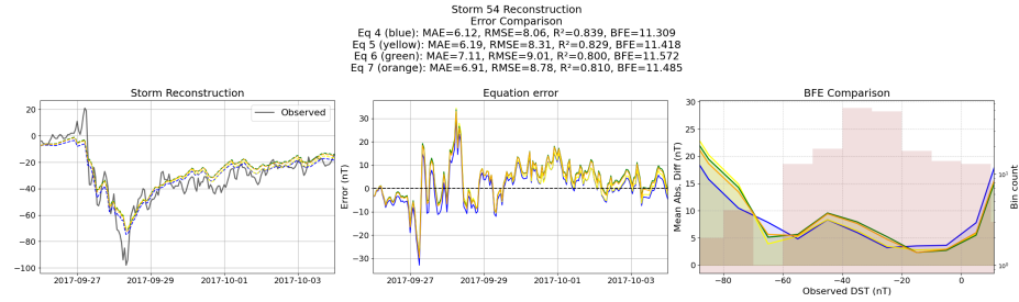
Figure 21: Reconstruction of storm 54 using the Equations generated from the unconstrained symbolic regression with the derived features
