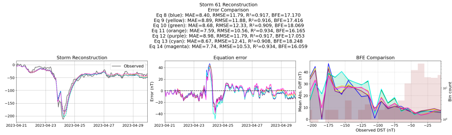
Figure 48: Reconstruction of storm 61 using the Equations generated from the templated symbolic regression with the primitive features
