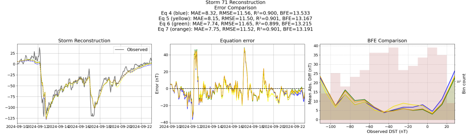
Figure 38: Reconstruction of storm 71 using the Equations generated from the unconstrained symbolic regression with the derived features
