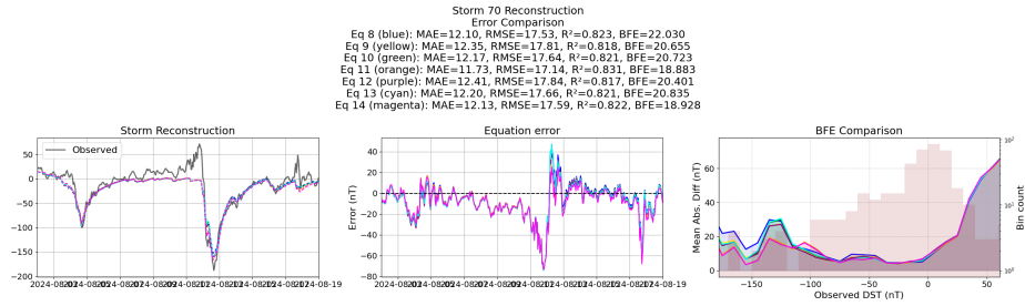
Figure 57: Reconstruction of storm 70 using the Equations generated from the templated symbolic regression with the primitive features
