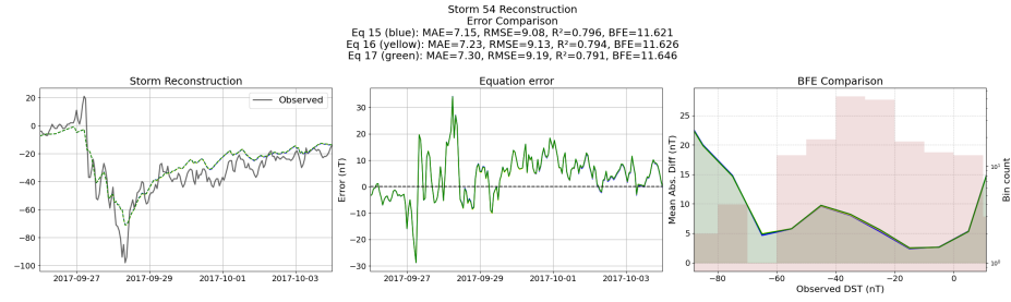
Figure 61: Reconstruction of storm 54 using the Equations generated from the templated symbolic regression with the derived features
