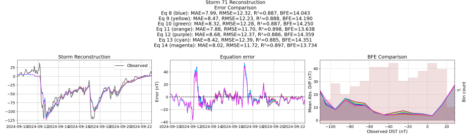
Figure 58: Reconstruction of storm 71 using the Equations generated from the templated symbolic regression with the primitive features
