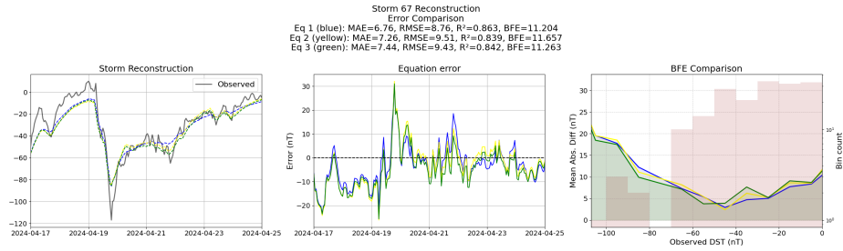
Figure 14: Reconstruction of storm 67 using the Equations generated from the unconstrained symbolic regression with the primitive features
