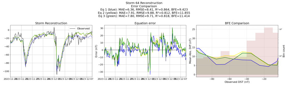
Figure 11: Reconstruction of storm 64 using the Equations generated from the unconstrained symbolic regression with the primitive features
