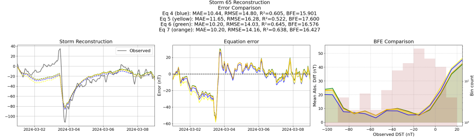
Figure 32: Reconstruction of storm 65 using the Equations generated from the unconstrained symbolic regression with the derived features
