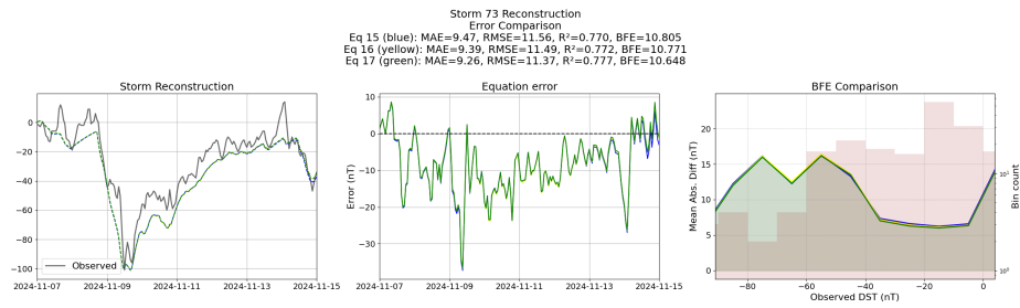
Figure 80: Reconstruction of storm 73 using the Equations generated from the templated symbolic regression with the derived features
