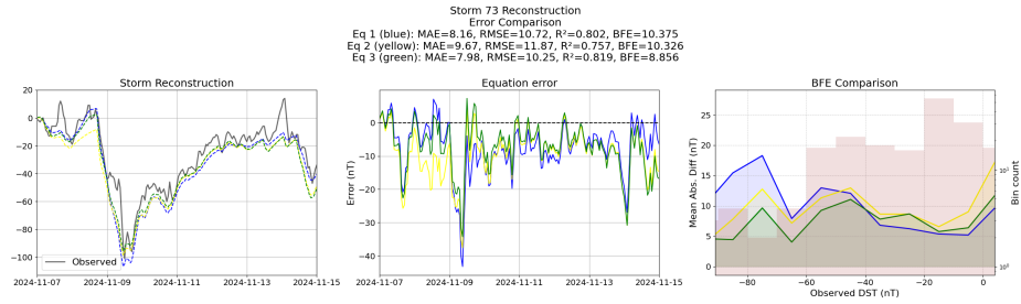
Figure 20: Reconstruction of storm 73 using the Equations generated from the unconstrained symbolic regression with the primitive features
