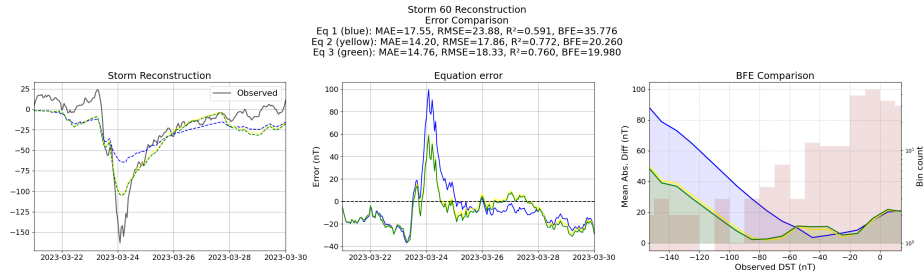
Figure 7: Reconstruction of storm 60 using the Equations generated from the unconstrained symbolic regression with the primitive features
