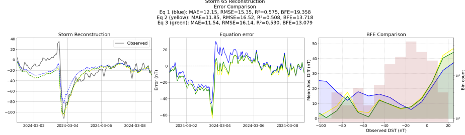
Figure 12: Reconstruction of storm 65 using the Equations generated from the unconstrained symbolic regression with the primitive features
