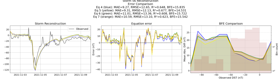
Figure 23: Reconstruction of storm 56 using the Equations generated from the unconstrained symbolic regression with the derived features
