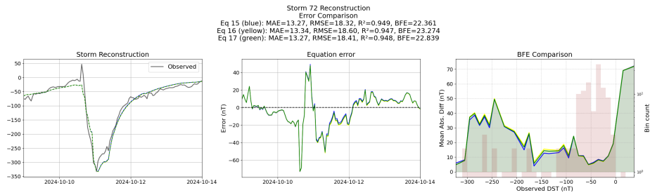
Figure 79: Reconstruction of storm 72 using the Equations generated from the templated symbolic regression with the derived features
