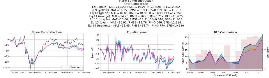
Figure 46: Reconstruction of storm 59 using the Equations generated from the templated symbolic regression with the primitive features
