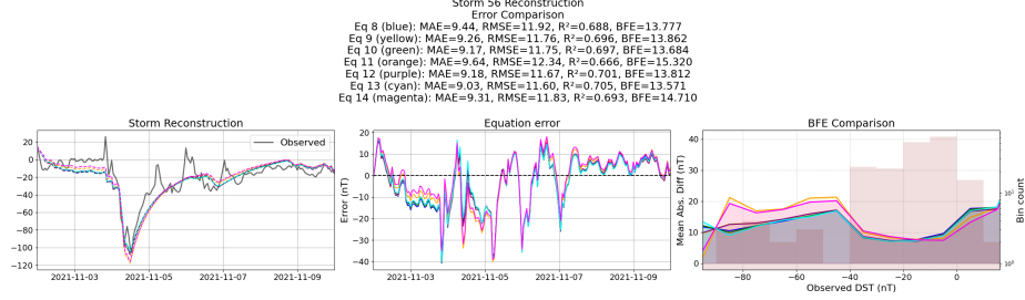
Figure 43: Reconstruction of storm 56 using the Equations generated from the templated symbolic regression with the primitive features
