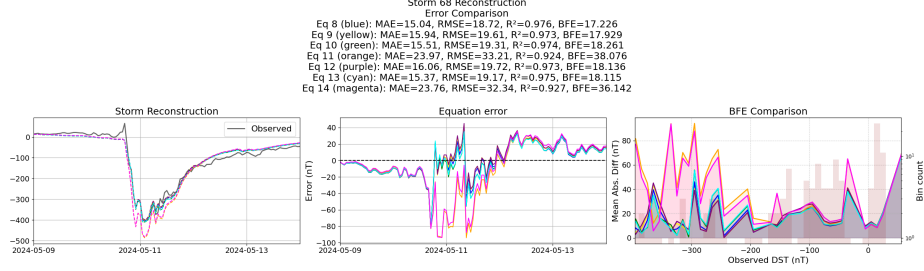
Figure 55: Reconstruction of storm 68 using the Equations generated from the templated symbolic regression with the primitive features
