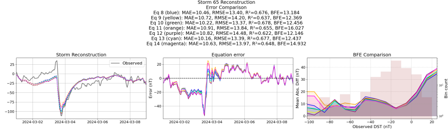
Figure 52: Reconstruction of storm 65 using the Equations generated from the templated symbolic regression with the primitive features
