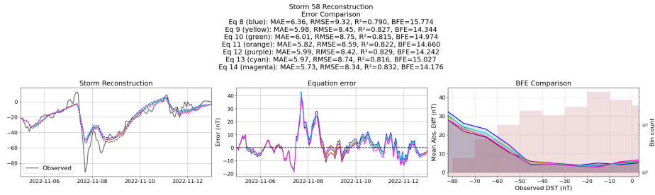
Figure 45: Reconstruction of storm 58 using the Equations generated from the templated symbolic regression with the primitive features
