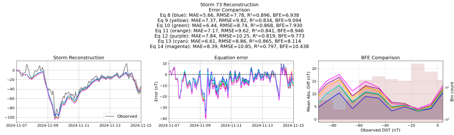
Figure 60: Reconstruction of storm 73 using the Equations generated from the templated symbolic regression with the primitive features
