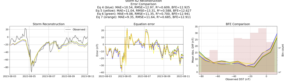
Figure 29: Reconstruction of storm 62 using the Equations generated from the unconstrained symbolic regression with the derived features
