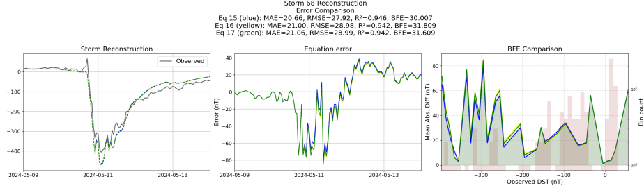
Figure 75: Reconstruction of storm 68 using the Equations generated from the templated symbolic regression with the derived features
