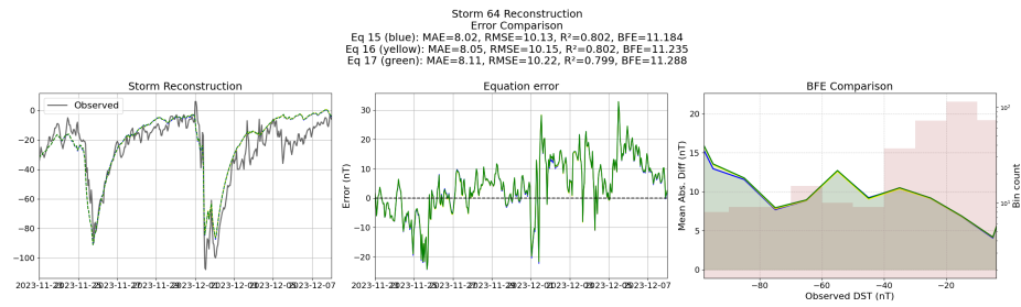
Figure 71: Reconstruction of storm 64 using the Equations generated from the templated symbolic regression with the derived features
