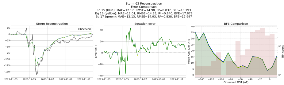
Figure 70: Reconstruction of storm 63 using the Equations generated from the templated symbolic regression with the derived features
