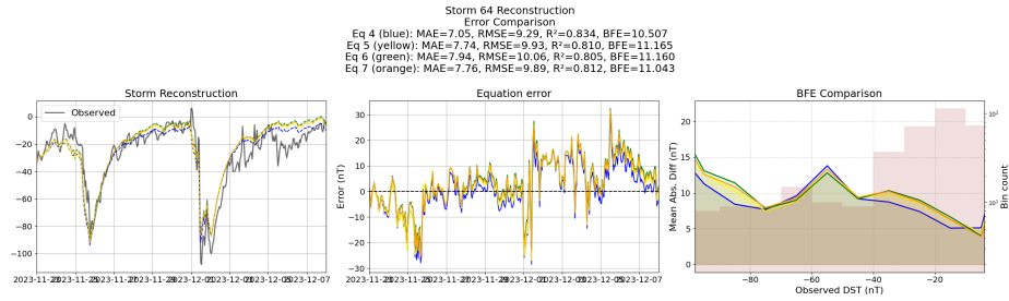
Figure 31: Reconstruction of storm 64 using the Equations generated from the unconstrained symbolic regression with the derived features
