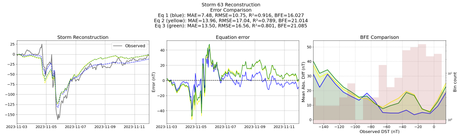
Figure 10: Reconstruction of storm 63 using the Equations generated from the unconstrained symbolic regression with the primitive features
