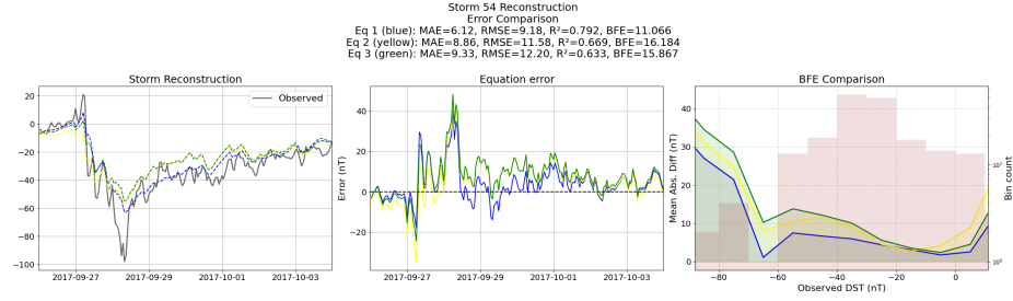
Figure 1: Reconstruction of storm 54 using the Equations generated from the unconstrained symbolic regression with the primitive features
