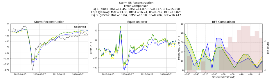
Figure 2: Reconstruction of storm 55 using the Equations generated from the unconstrained symbolic regression with the primitive features
