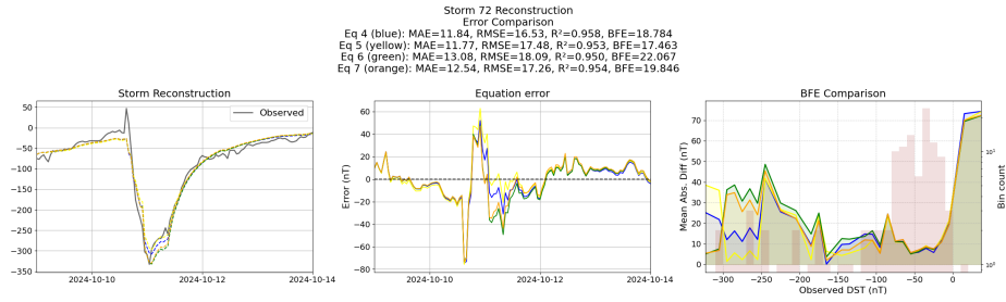
Figure 39: Reconstruction of storm 72 using the Equations generated from the unconstrained symbolic regression with the derived features
