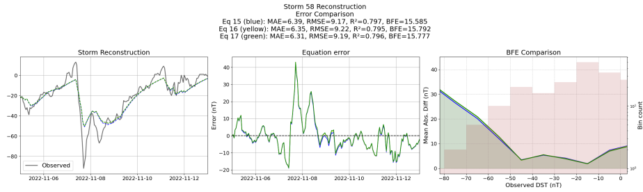
Figure 65: Reconstruction of storm 58 using the Equations generated from the templated symbolic regression with the derived features
