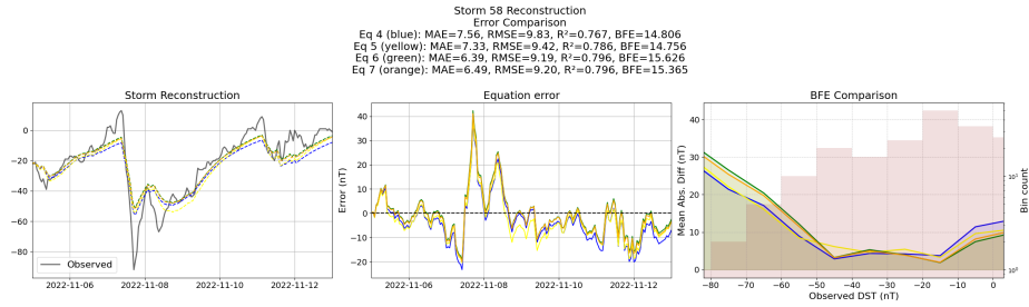
Figure 25: Reconstruction of storm 58 using the Equations generated from the unconstrained symbolic regression with the derived features
