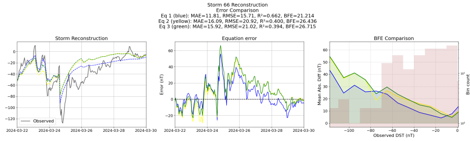
Figure 13: Reconstruction of storm 66 using the Equations generated from the unconstrained symbolic regression with the primitive features
