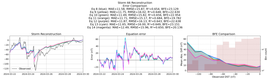
Figure 53: Reconstruction of storm 66 using the Equations generated from the templated symbolic regression with the primitive features
