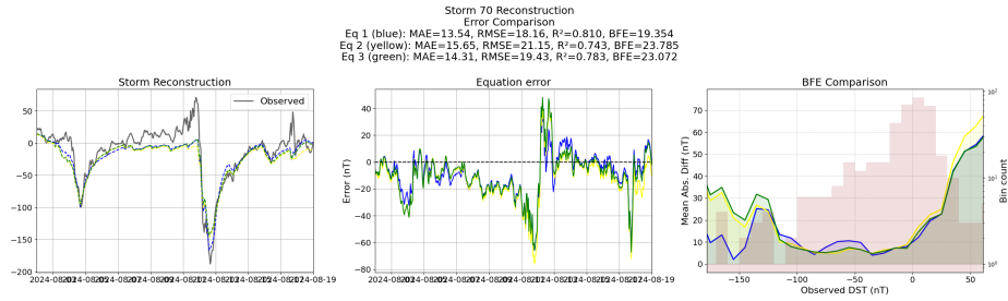
Figure 17: Reconstruction of storm 70 using the Equations generated from the unconstrained symbolic regression with the primitive features
