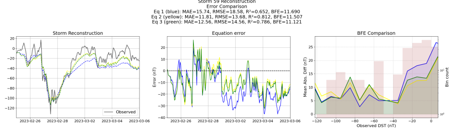
Figure 6: Reconstruction of storm 59 using the Equations generated from the unconstrained symbolic regression with the primitive features
