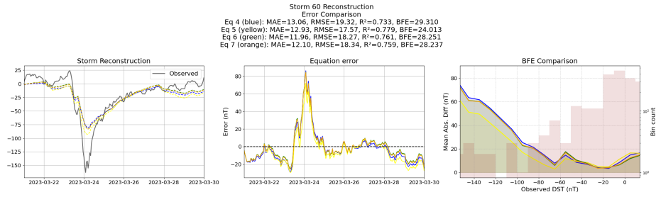
Figure 27: Reconstruction of storm 60 using the Equations generated from the unconstrained symbolic regression with the derived features
