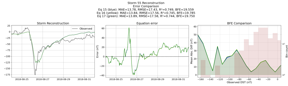
Figure 62: Reconstruction of storm 55 using the Equations generated from the templated symbolic regression with the derived features
