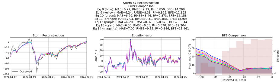
Figure 54: Reconstruction of storm 67 using the Equations generated from the templated symbolic regression with the primitive features
