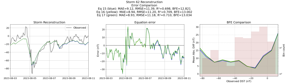
Figure 69: Reconstruction of storm 62 using the Equations generated from the templated symbolic regression with the derived features
