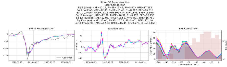
Figure 42: Reconstruction of storm 55 using the Equations generated from the templated symbolic regression with the primitive features
