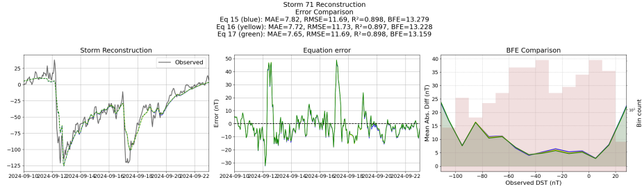
Figure 78: Reconstruction of storm 71 using the Equations generated from the templated symbolic regression with the derived features
