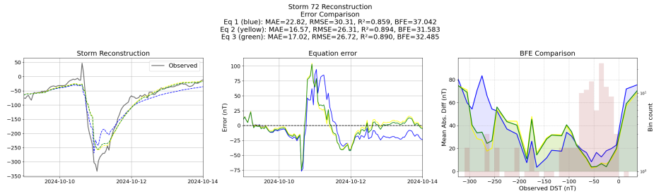
Figure 19: Reconstruction of storm 72 using the Equations generated from the unconstrained symbolic regression with the primitive features
