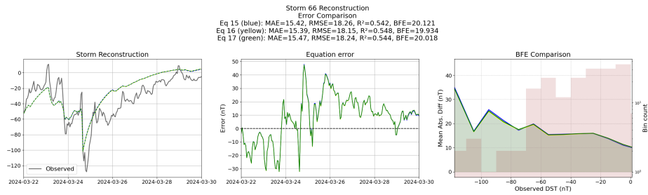
Figure 73: Reconstruction of storm 66 using the Equations generated from the templated symbolic regression with the derived features
