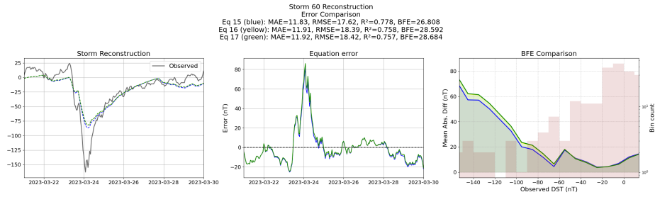
Figure 67: Reconstruction of storm 60 using the Equations generated from the templated symbolic regression with the derived features
