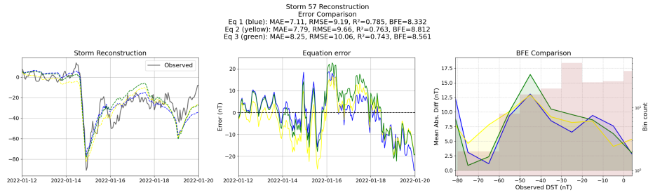
Figure 4: Reconstruction of storm 57 using the Equations generated from the unconstrained symbolic regression with the primitive features
