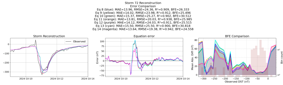
Figure 59: Reconstruction of storm 72 using the Equations generated from the templated symbolic regression with the primitive features
