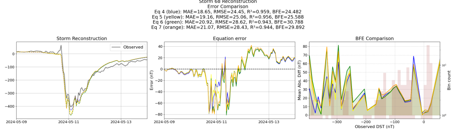
Figure 35: Reconstruction of storm 68 using the Equations generated from the unconstrained symbolic regression with the derived features
