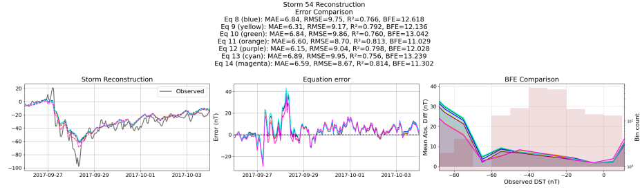
Figure 41: Reconstruction of storm 54 using the Equations generated from the templated symbolic regression with the primitive features
