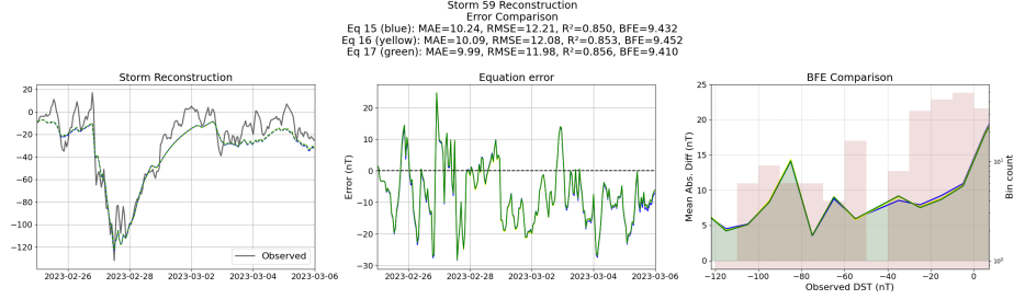
Figure 66: Reconstruction of storm 59 using the Equations generated from the templated symbolic regression with the derived features
