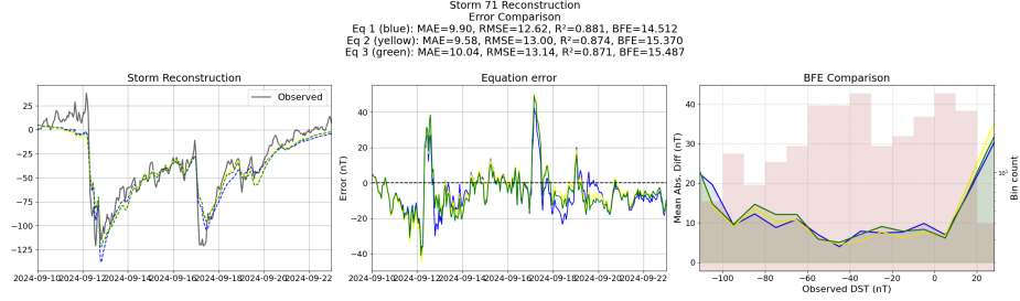
Figure 18: Reconstruction of storm 71 using the Equations generated from the unconstrained symbolic regression with the primitive features
