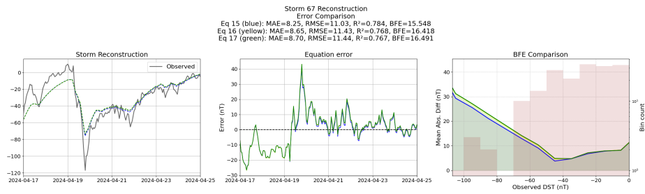
Figure 74: Reconstruction of storm 67 using the Equations generated from the templated symbolic regression with the derived features
