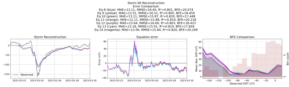
Figure 47: Reconstruction of storm 60 using the Equations generated from the templated symbolic regression with the primitive features
