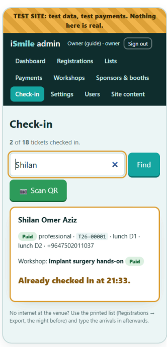
Scanned again: already checked in.
