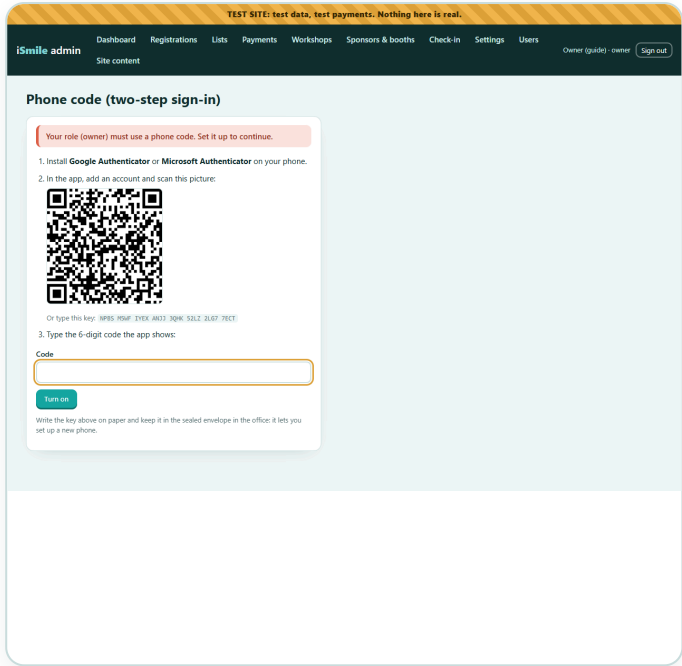
Steps 2–3: scan the picture, type the 6-digit code. (This is a test account; your picture will be different.)
