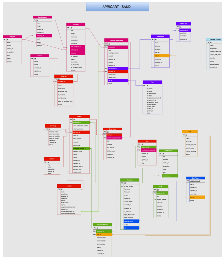
Figure 1: Entity-Relationship Diagram - ERD
