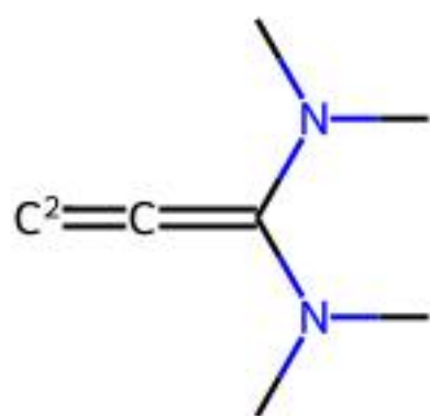
UDODAU | ILP unmatched ligand(s) | ox=2
