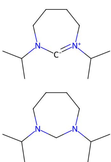
TIZKIY | ILP unmatched ligand(s) | ox=0
