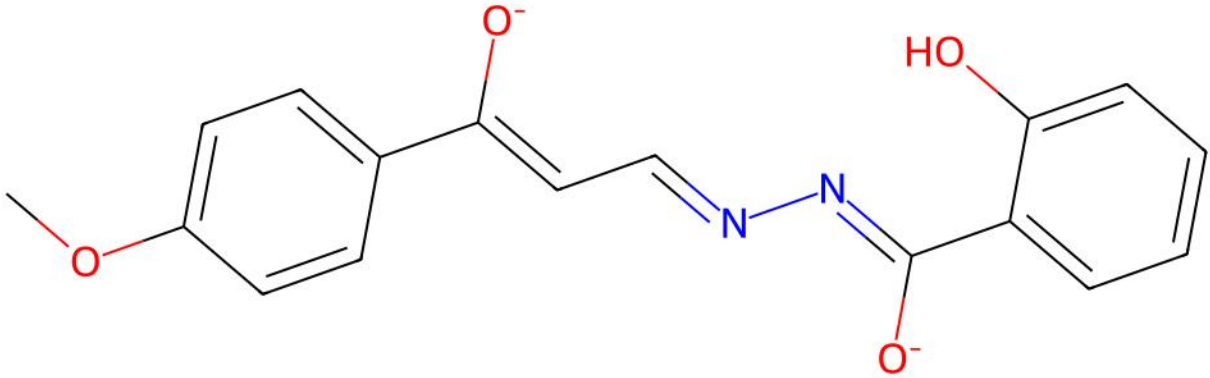
UXOJEY | Reference unmatched ligand(s)
