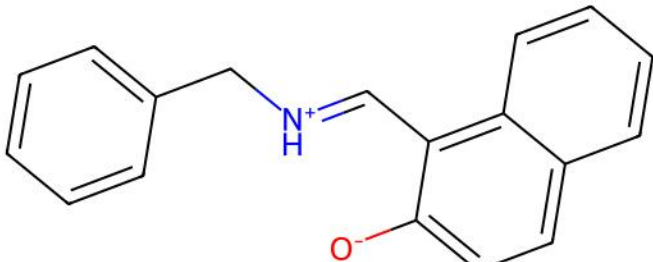
AQEXIE | ILP unmatched ligand(s) | ox=0
