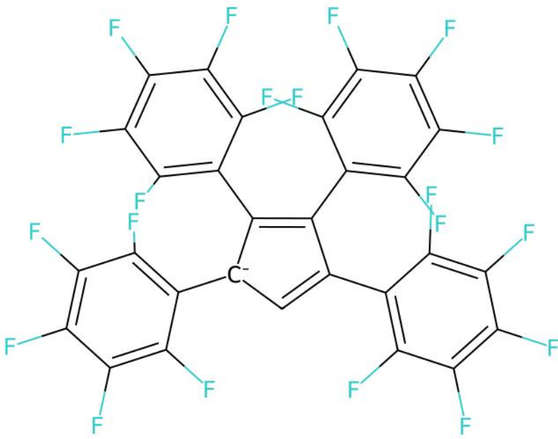
MICRUL | Reference unmatched ligand(s)
