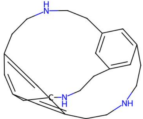
PUJNIR | Reference unmatched ligand(s)
