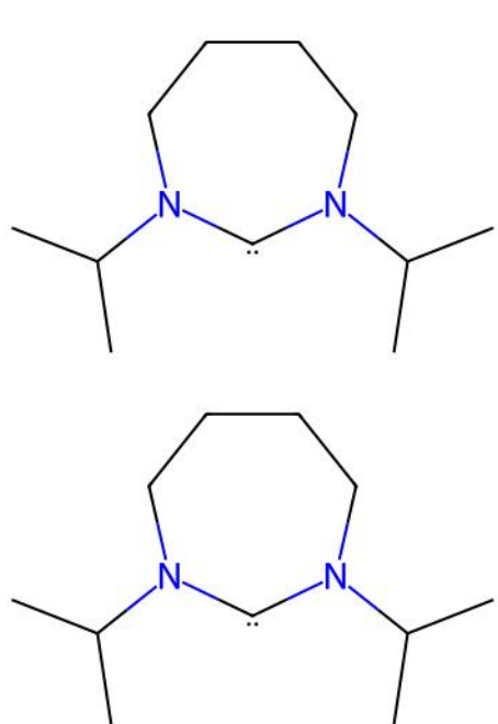
TIZKIY | Reference unmatched ligand(s)
