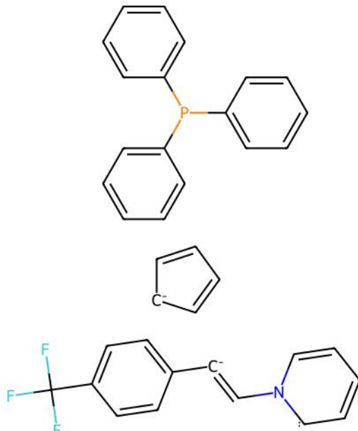
CIFPUE | Reference unmatched ligand(s)
