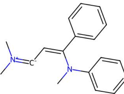
FIRFES | ILP unmatched ligand(s) | ox=0
