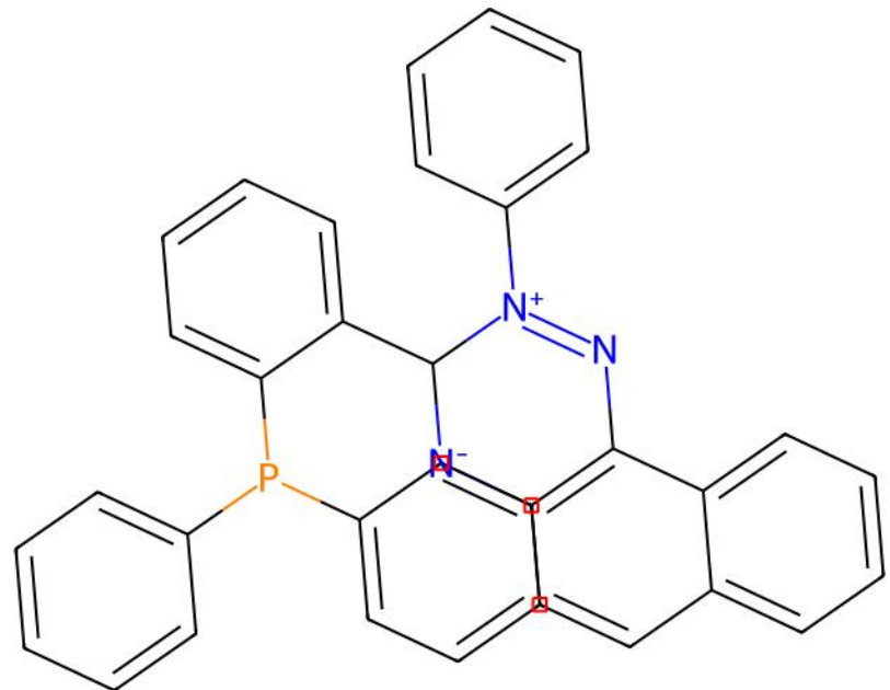
INUDAW | ILP unmatched ligand(s) | ox=0
