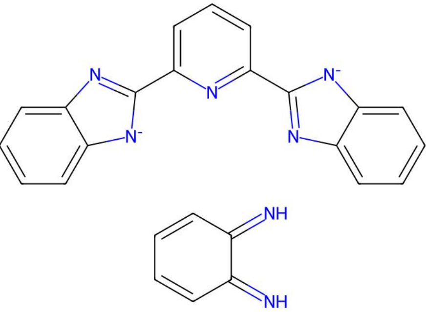
SOMNEO | Reference unmatched ligand(s)
