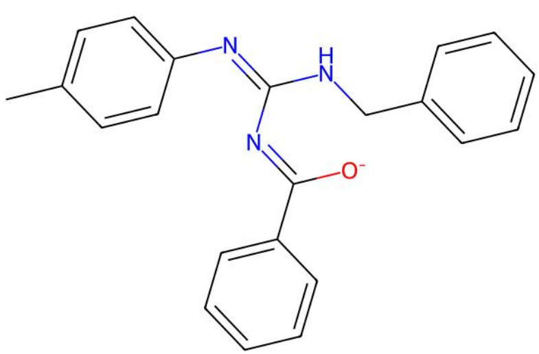
TOBNEG | Reference unmatched ligand(s)
