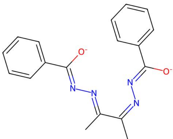
KUBFIX | Reference unmatched ligand(s)
