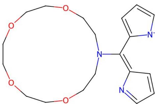
KAHNOZ | Reference unmatched ligand(s)
