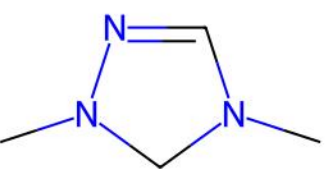
HUPGOQ | ILP unmatched ligand(s) | ox=-2
