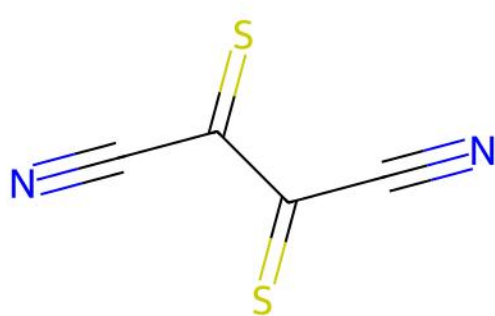
WELWIT | ILP unmatched ligand(s) | ox=-2
