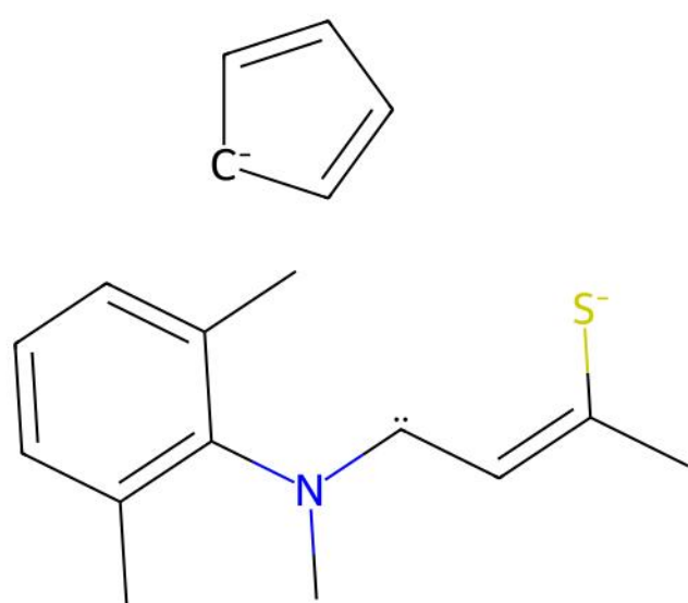
WEQCOL | Reference unmatched ligand(s)
