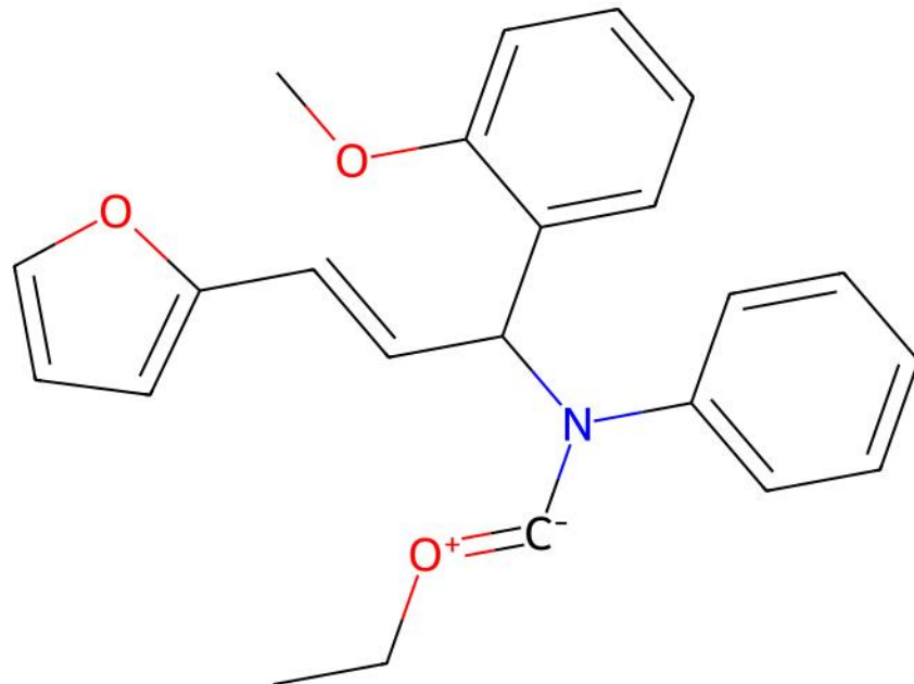
FACBIV | ILP unmatched ligand(s) | ox=0
