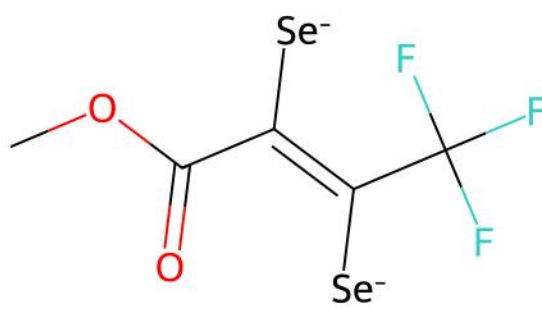
XIKGII | Reference unmatched ligand(s)
