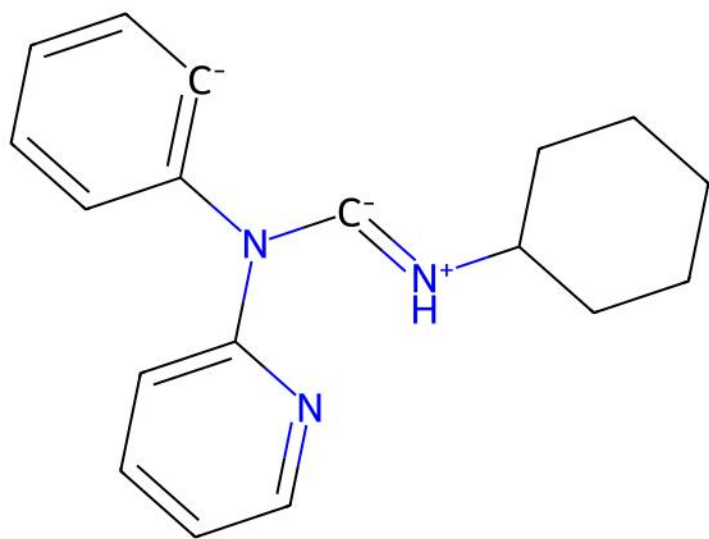
XIRFIP | ILP unmatched ligand(s) | ox=0
