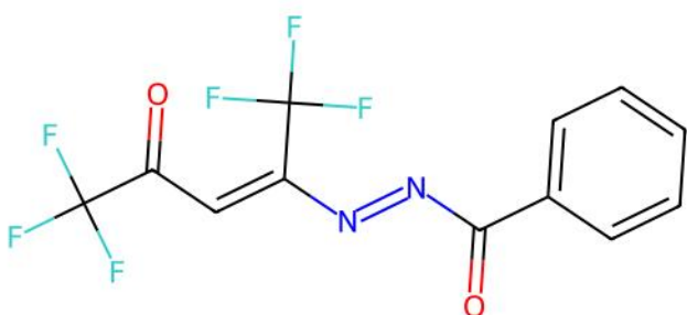
LUMNIS | ILP unmatched ligand(s) | ox=-2
