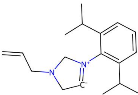
PIKPEG | ILP unmatched ligand(s) | ox=0
