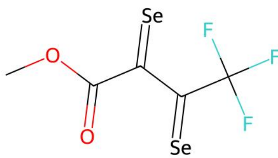
XIKGII | ILP unmatched ligand(s) | ox=-2
