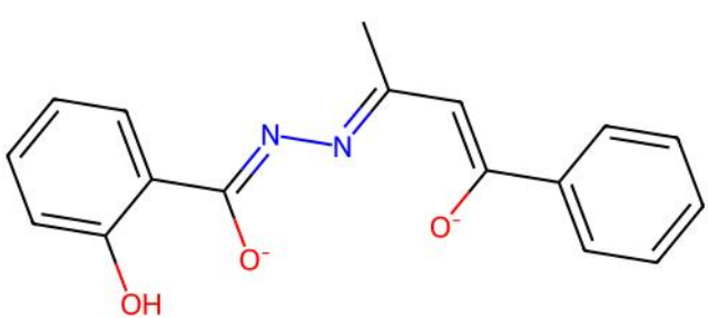
YODHEE | Reference unmatched ligand(s)
