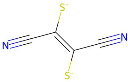
PIDCAJ | Reference unmatched ligand(s)
