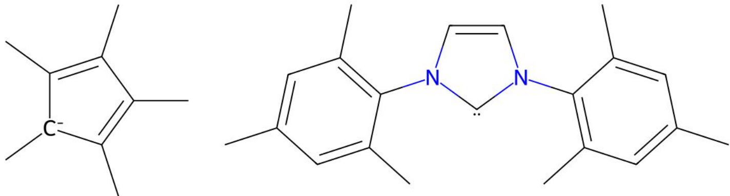
FAJDAW | Reference unmatched ligand(s)
