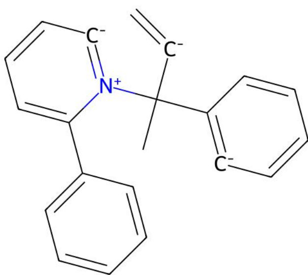
FETHET | ILP unmatched ligand(s) | ox=0
