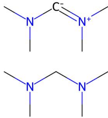
XOMFIR | ILP unmatched ligand(s) | ox=0
