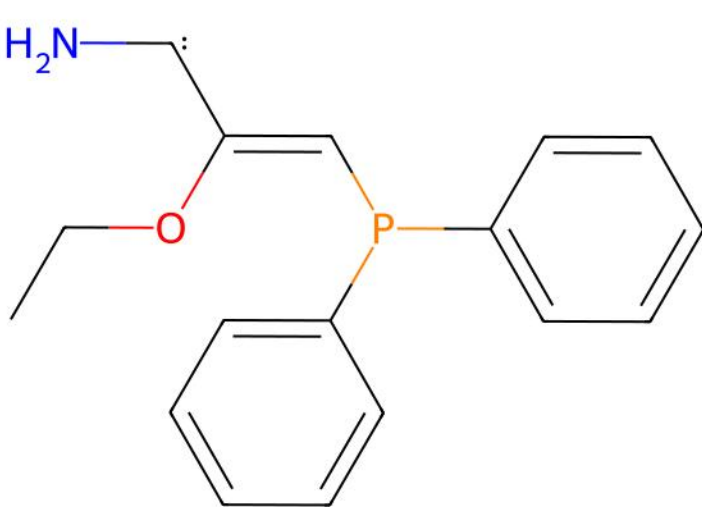
FIHNEP | Reference unmatched ligand(s)
