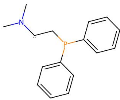
FINTIG | Reference unmatched ligand(s)
