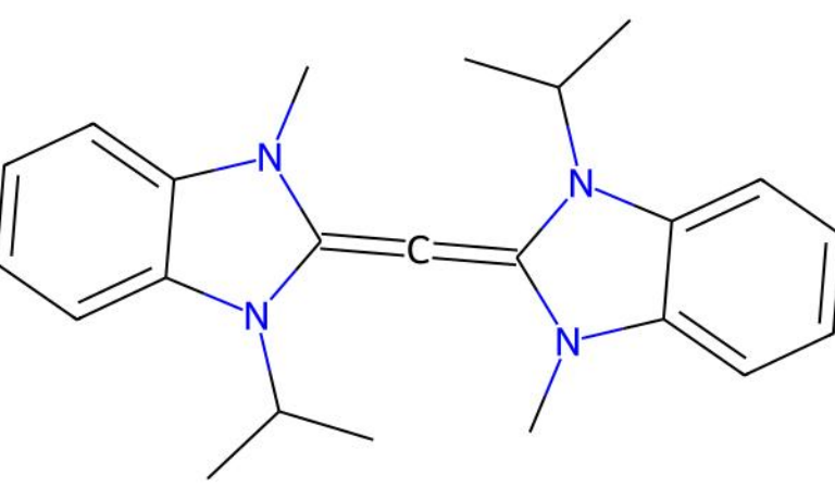
SIFCER | Reference unmatched ligand(s)
