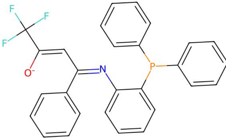
KAWTEJ | Reference unmatched ligand(s)
