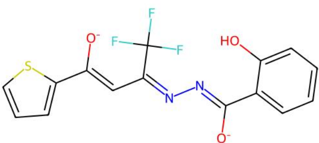
YODHAA | Reference unmatched ligand(s)
