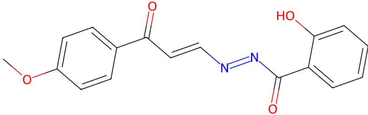
UXOJEY | ILP unmatched ligand(s) | ox=-2
