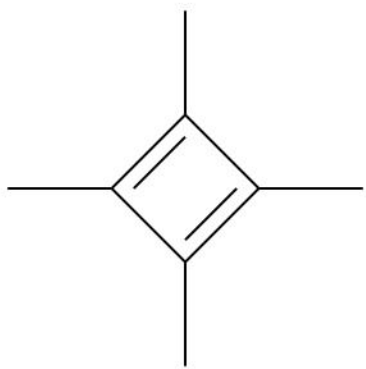
URUKUO | Reference unmatched ligand(s)
