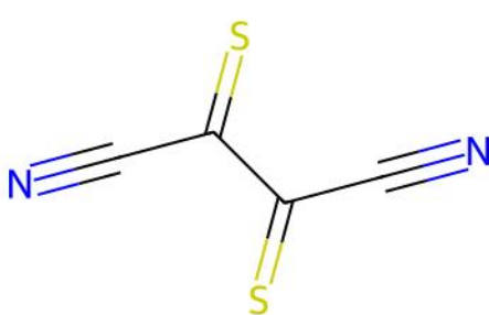
ICEGOO | ILP unmatched ligand(s) | ox=-2
