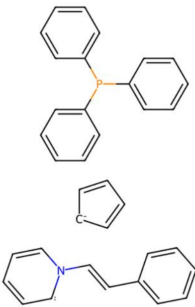
CIFQEP | Reference unmatched ligand(s)
