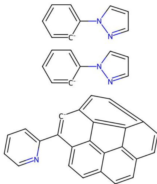
YUCHEL | Reference unmatched ligand(s)
