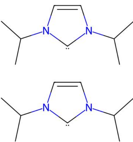
SOKSES | Reference unmatched ligand(s)
