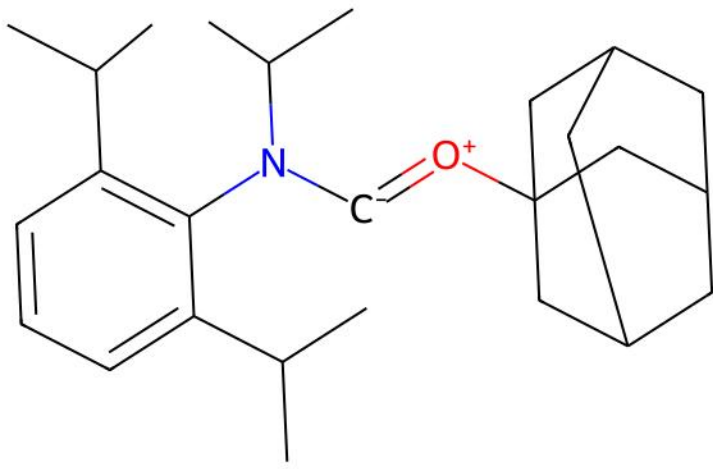
PEKMOJ | ILP unmatched ligand(s) | ox=0
