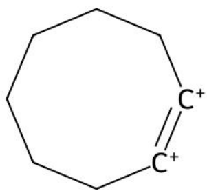
XAGNOI | ILP unmatched ligand(s) | ox=-2
