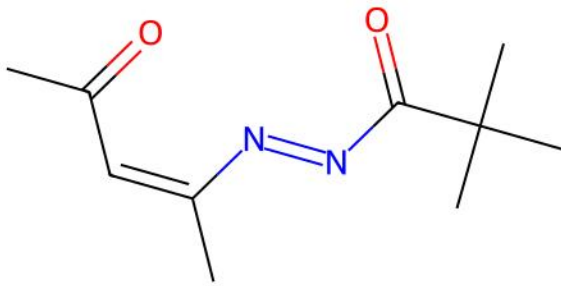
MUFHEC | ILP unmatched ligand(s) | ox=-2
