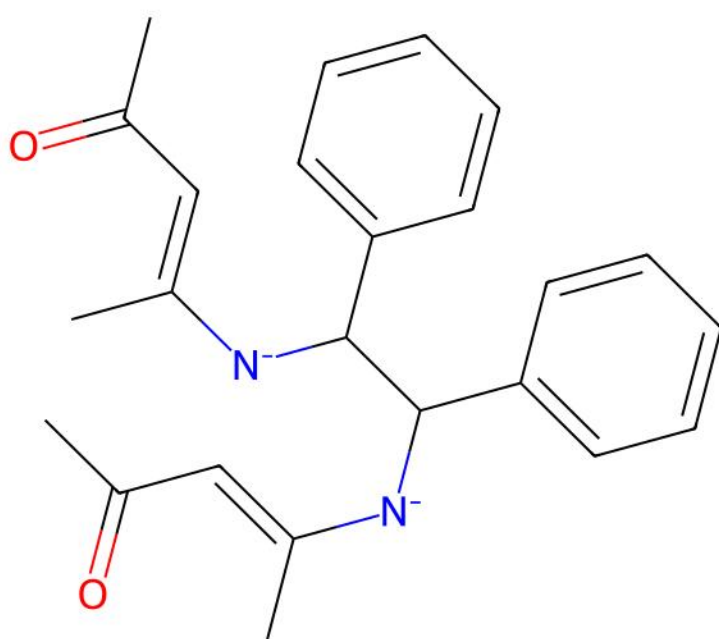
UNAVOW | ILP unmatched ligand(s) | ox=0
