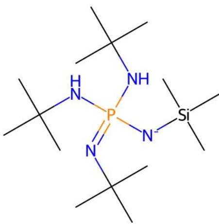
MIJQIG | ILP unmatched ligand(s) | ox=0
