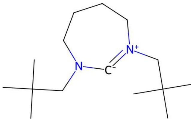
XIWYAG | ILP unmatched ligand(s) | ox=0
