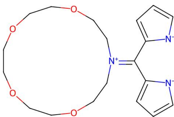
KAHNOZ | ILP unmatched ligand(s) | ox=0
