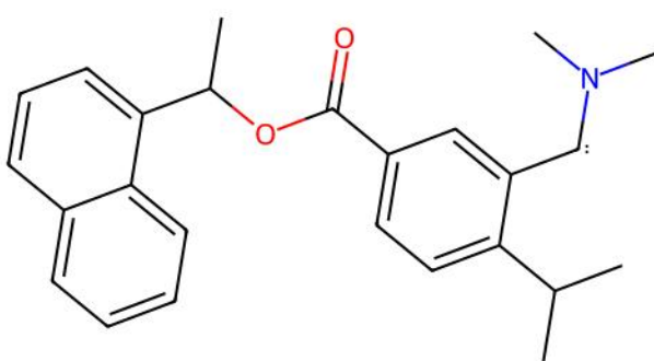
YIYCOZ | Reference unmatched ligand(s)
