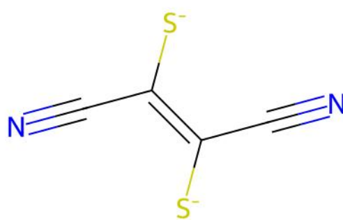
WELWOZ | Reference unmatched ligand(s)
