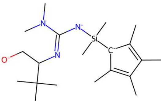
YOBTAL | Reference unmatched ligand(s)
