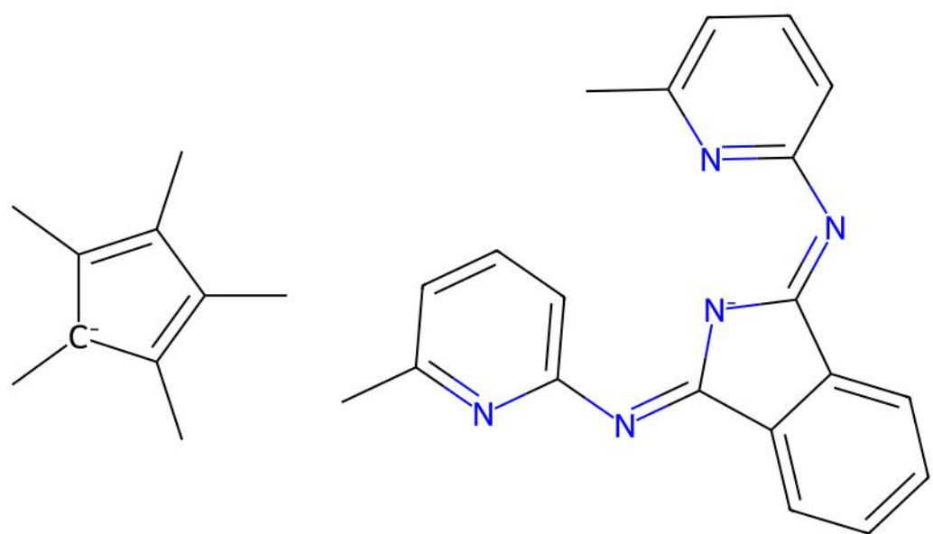
HUPGOQ | Reference unmatched ligand(s)
