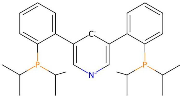
MUTSEB | ILP unmatched ligand(s) | ox=2
