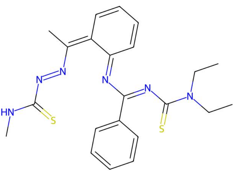
TULRAV | ILP unmatched ligand(s) | ox=-2
