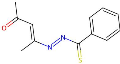
POQSAP | ILP unmatched ligand(s) | ox=-2
