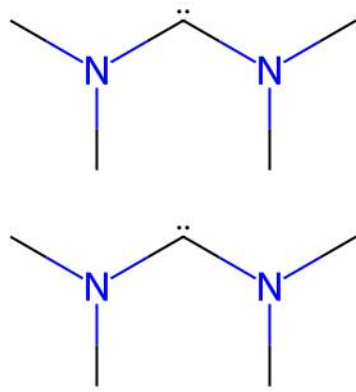
XOMFIR | Reference unmatched ligand(s)
