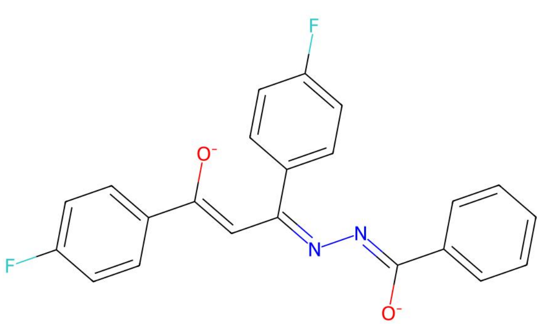
VOYWIP | Reference unmatched ligand(s)
