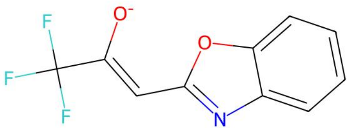
PIGBIT | Reference unmatched ligand(s)
