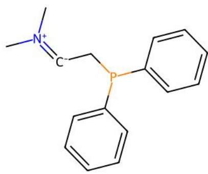
FINTIG | ILP unmatched ligand(s) | ox=0
