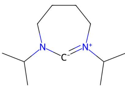
XIWXUZ | ILP unmatched ligand(s) | ox=0
