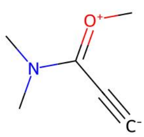
UDOCAT | ILP unmatched ligand(s) | ox=0
