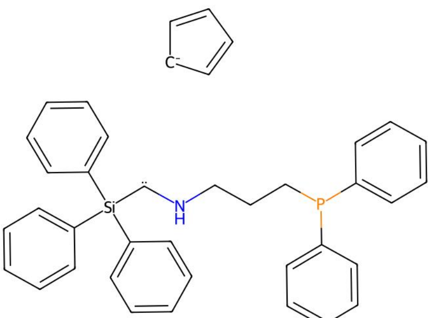
AMINOA | Reference unmatched ligand(s)
