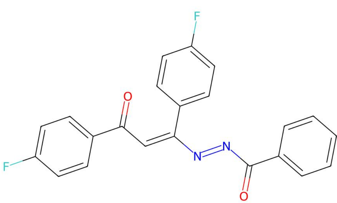
VOYWIP | ILP unmatched ligand(s) | ox=-2
