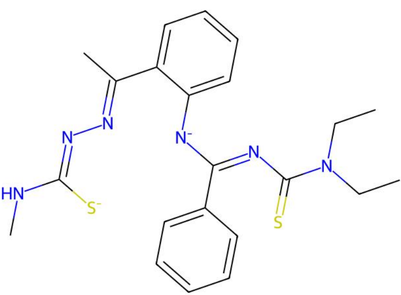
TULRAV | Reference unmatched ligand(s)
