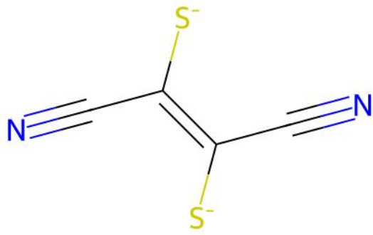
FEVYEL | Reference unmatched ligand(s)
