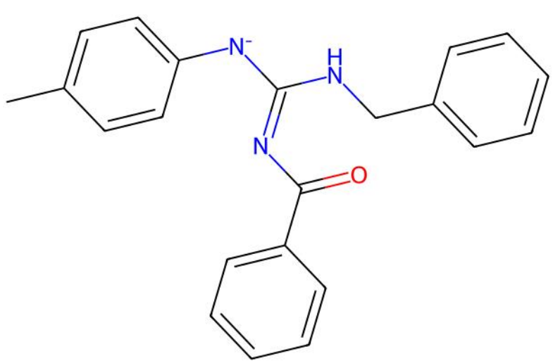
TOBNEG | ILP unmatched ligand(s) | ox=0
