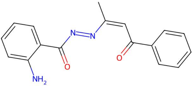
ACUKOB | ILP unmatched ligand(s) | ox=-2
