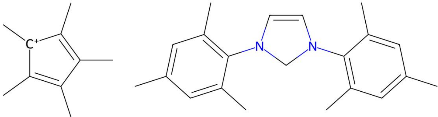
FAJDAW | ILP unmatched ligand(s) | ox=-2
