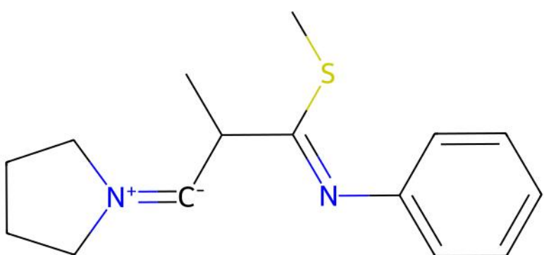
WEHFEW | ILP unmatched ligand(s) | ox=0
