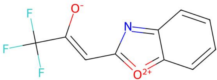
PIGBIT | ILP unmatched ligand(s) | ox=-2
