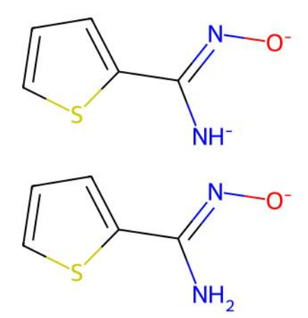
RASBIW | Reference unmatched ligand(s)
