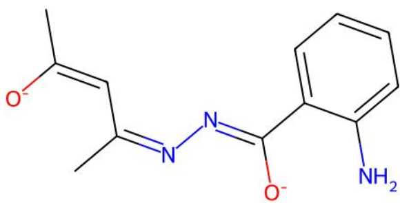
ACUJUG | Reference unmatched ligand(s)
