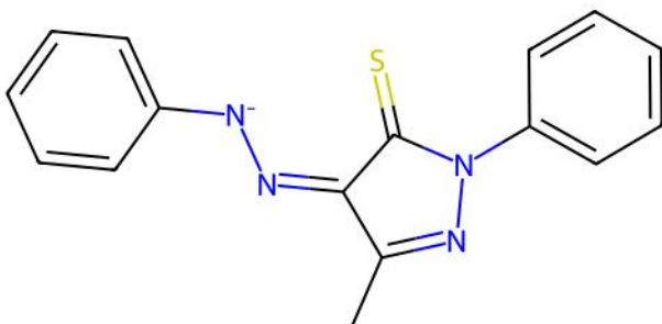
PILPUV | Reference unmatched ligand(s)
