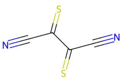
TUGTIY | ILP unmatched ligand(s) | ox=-2
