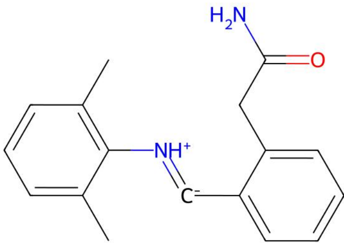
EPOMUS | ILP unmatched ligand(s) | ox=0
