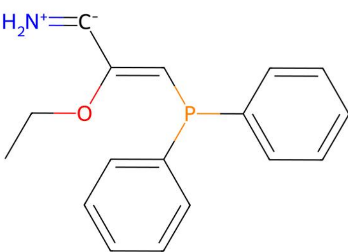
FIHNEP | ILP unmatched ligand(s) | ox=0
