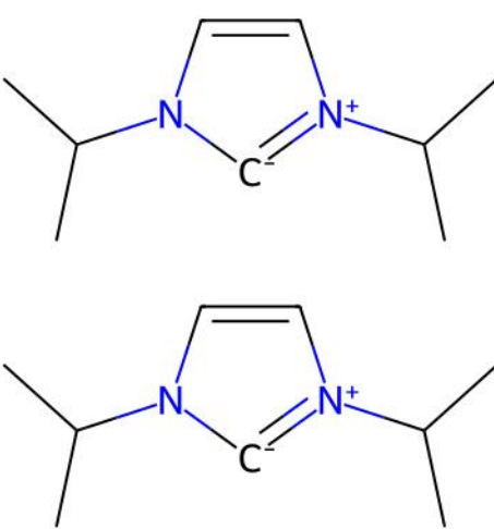
SOKSES | ILP unmatched ligand(s) | ox=0
