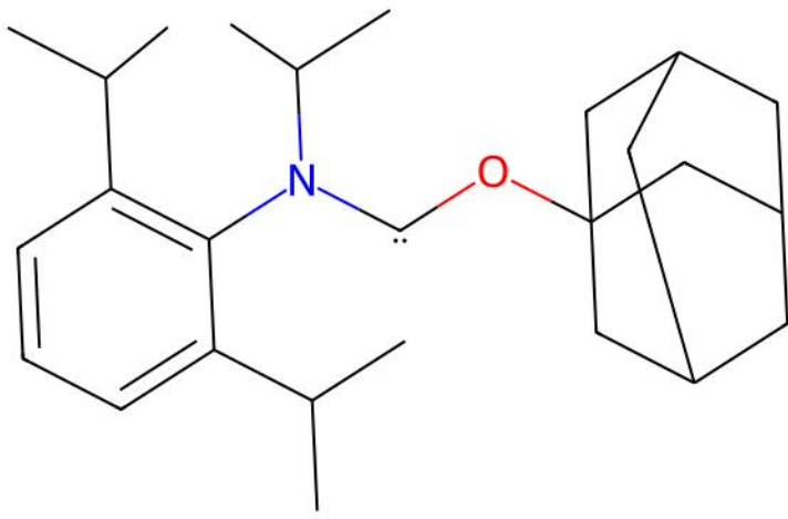
PEKMOJ | Reference unmatched ligand(s)
