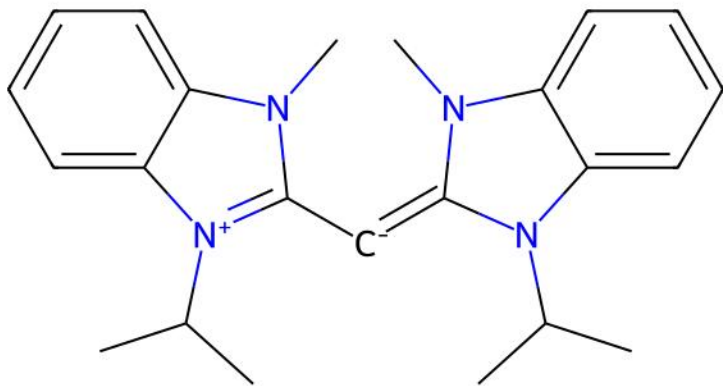
SIFCER | ILP unmatched ligand(s) | ox=0
