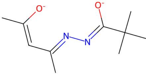
MUFHEC | Reference unmatched ligand(s)
