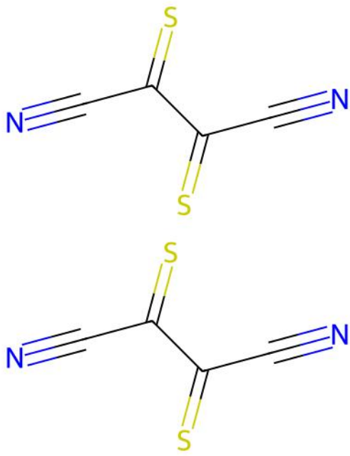
PCESMO | ILP unmatched ligand(s) | ox=-4
