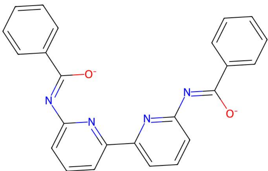
EFINUC | Reference unmatched ligand(s)
