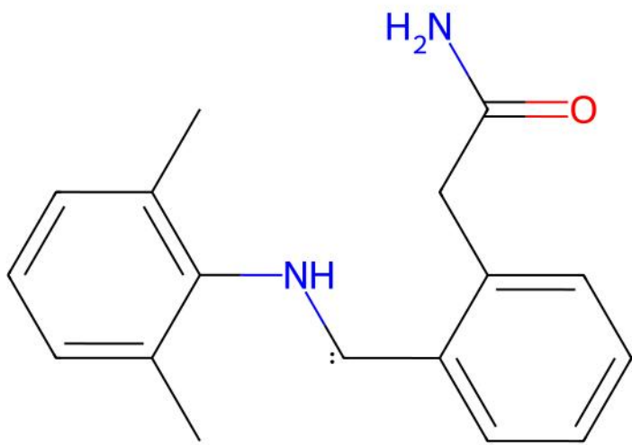
EPOMUS | Reference unmatched ligand(s)
