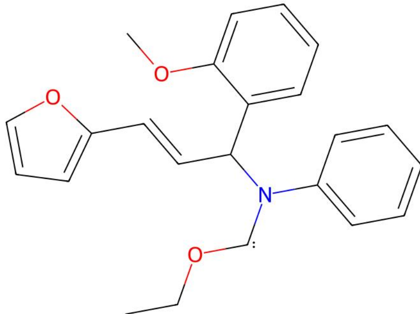
FACBIV | Reference unmatched ligand(s)
