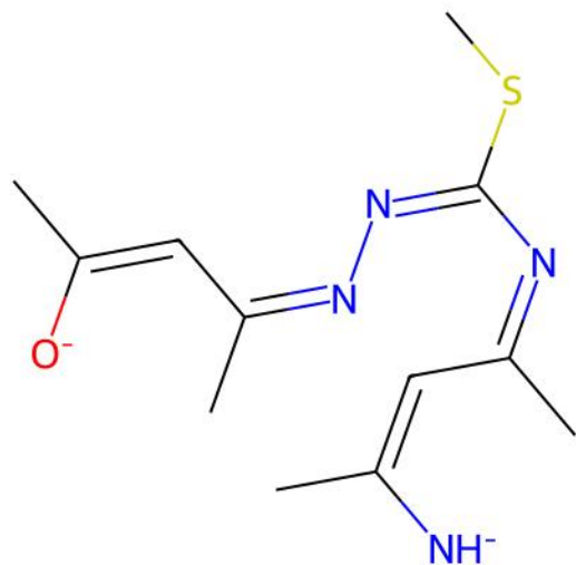
HUJVUD | Reference unmatched ligand(s)
