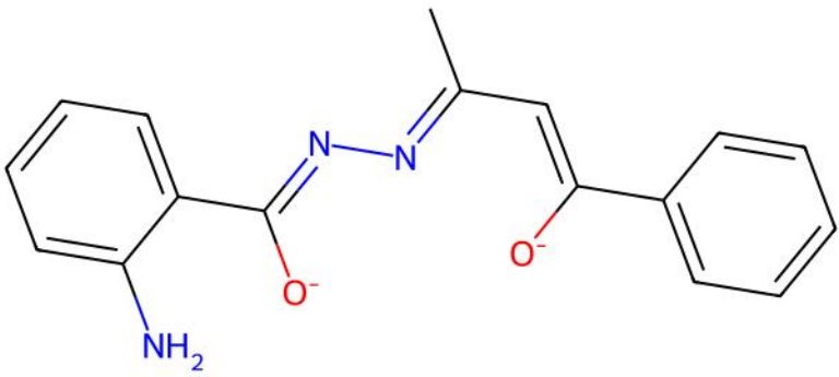
ACUKOB | Reference unmatched ligand(s)
