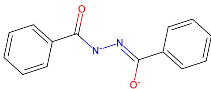
REHPID | Reference unmatched ligand(s)
