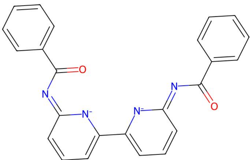
EFINUC | ILP unmatched ligand(s) | ox=0
