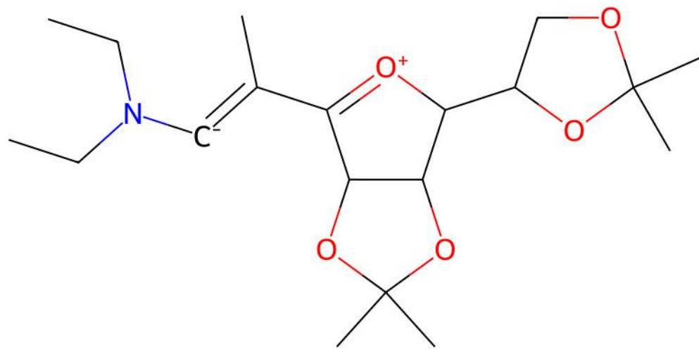
UNAMIF | ILP unmatched ligand(s) | ox=0
