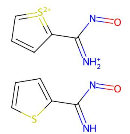
RASBIW | ILP unmatched ligand(s) | ox=-6
