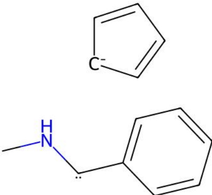
SIGFEV | Reference unmatched ligand(s)
