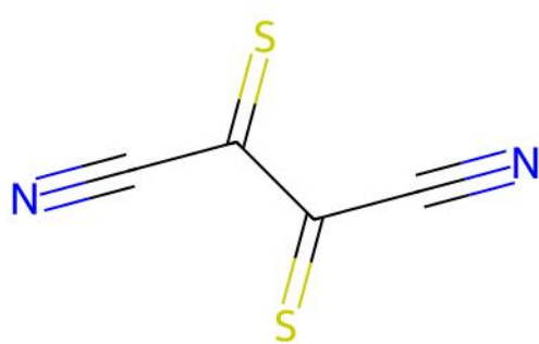
WEMTEP | ILP unmatched ligand(s) | ox=-2
