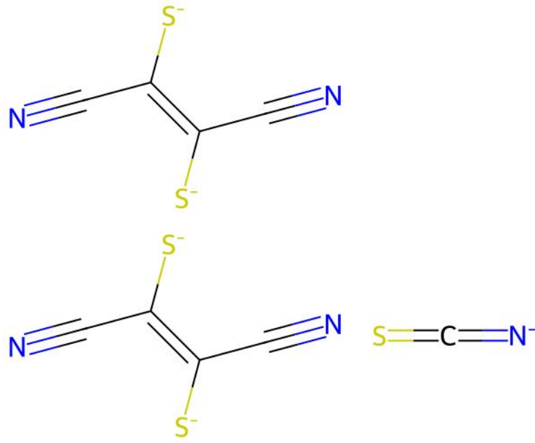
XOSRAZ | Reference unmatched ligand(s)
