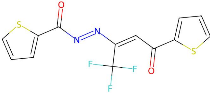
SOBKEB | ILP unmatched ligand(s) | ox=-2
