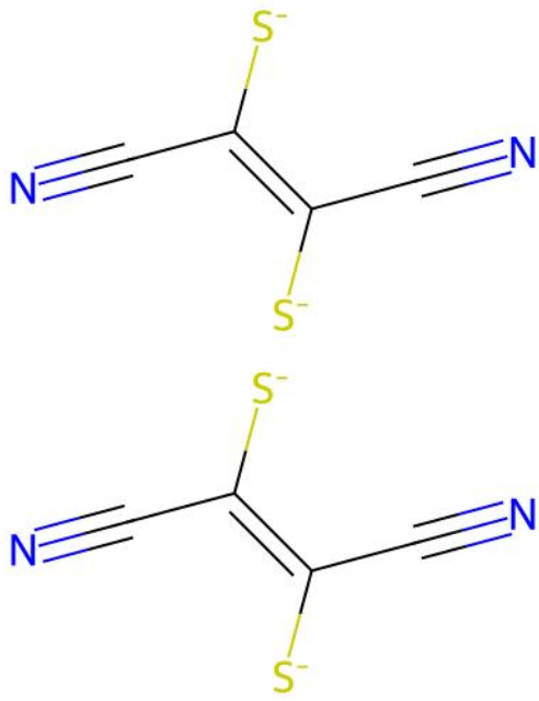
PCESMO | Reference unmatched ligand(s)
