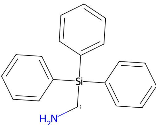
ESODEW | Reference unmatched ligand(s)
