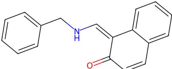
AQEXIE | Reference unmatched ligand(s)
