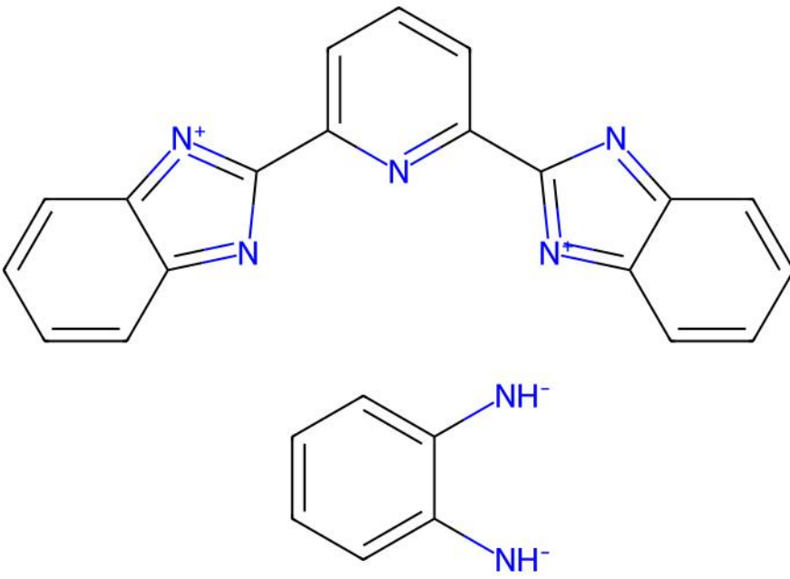
SOMNEO | ILP unmatched ligand(s) | ox=-2
