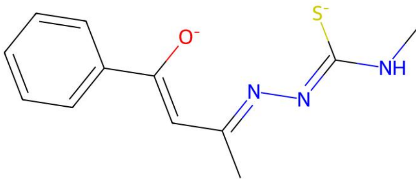
UMAPOP | Reference unmatched ligand(s)
