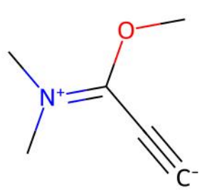
UDOBOG | Reference unmatched ligand(s)
