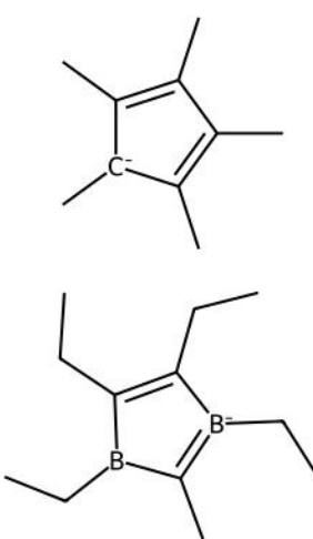
CEQRIZ | Reference unmatched ligand(s)
