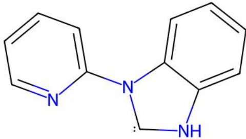
MIXQOC | Reference unmatched ligand(s)
