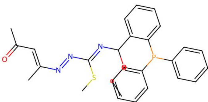
CELHAD | ILP unmatched ligand(s) | ox=-2
