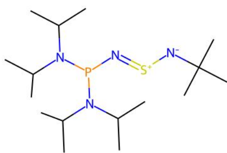
YUJPOI | ILP unmatched ligand(s) | ox=0
