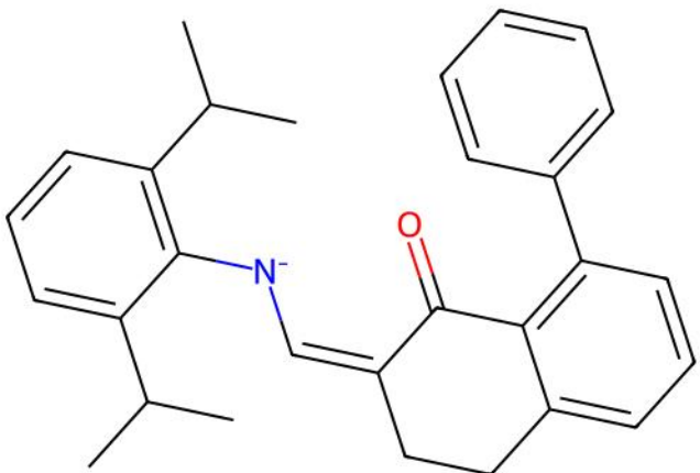
AQEXIE | ILP unmatched ligand(s) | ox=0
