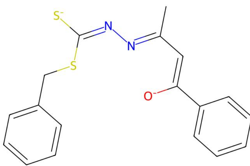
WAHBUE | Reference unmatched ligand(s)
