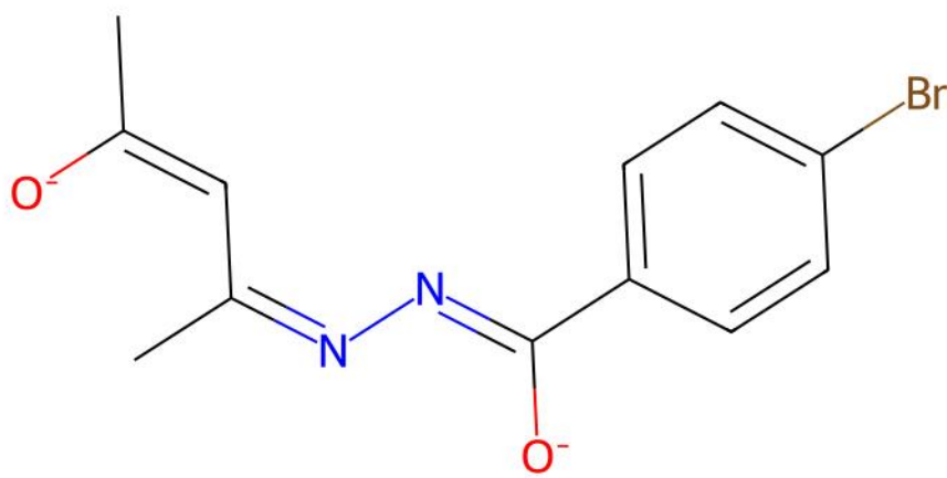
ULATUY | Reference unmatched ligand(s)
