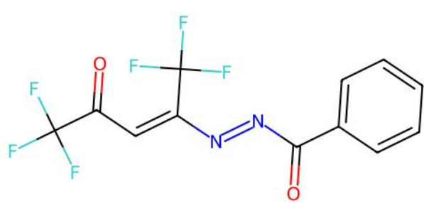
YOPKEV | ILP unmatched ligand(s) | ox=-2
