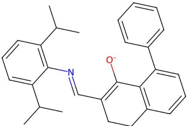
AQEXIE | Reference unmatched ligand(s)
