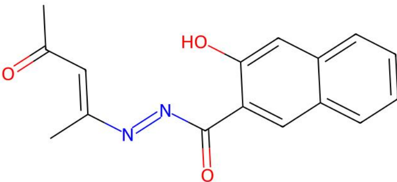
DURREO | ILP unmatched ligand(s) | ox=-2
