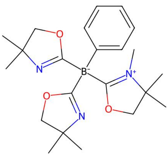
TUHRAQ | Reference unmatched ligand(s)
