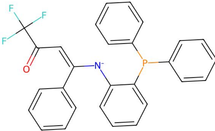
KAWTEJ | ILP unmatched ligand(s) | ox=0
