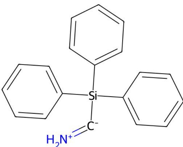
ESODEW | ILP unmatched ligand(s) | ox=0
