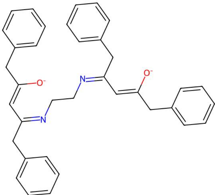
MAMVAX | Reference unmatched ligand(s)
