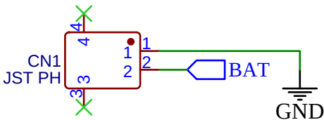
Battery Connection
