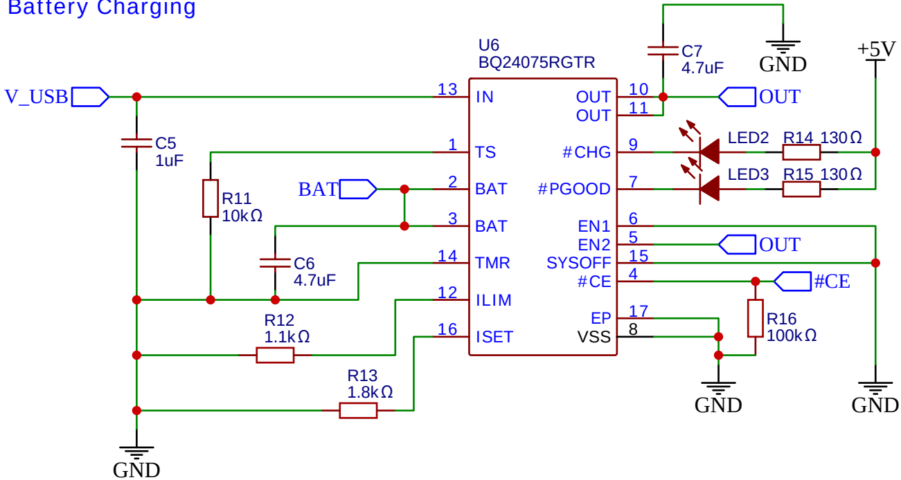
Battery Charging
