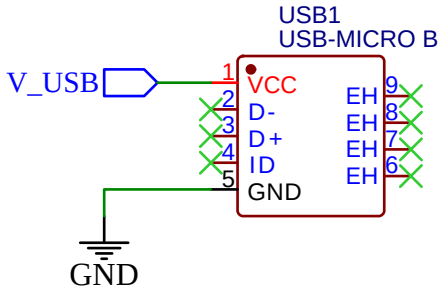
USB Power Connection
