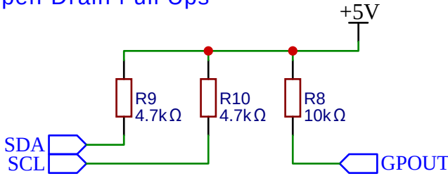
Open Drain Pull Ups
