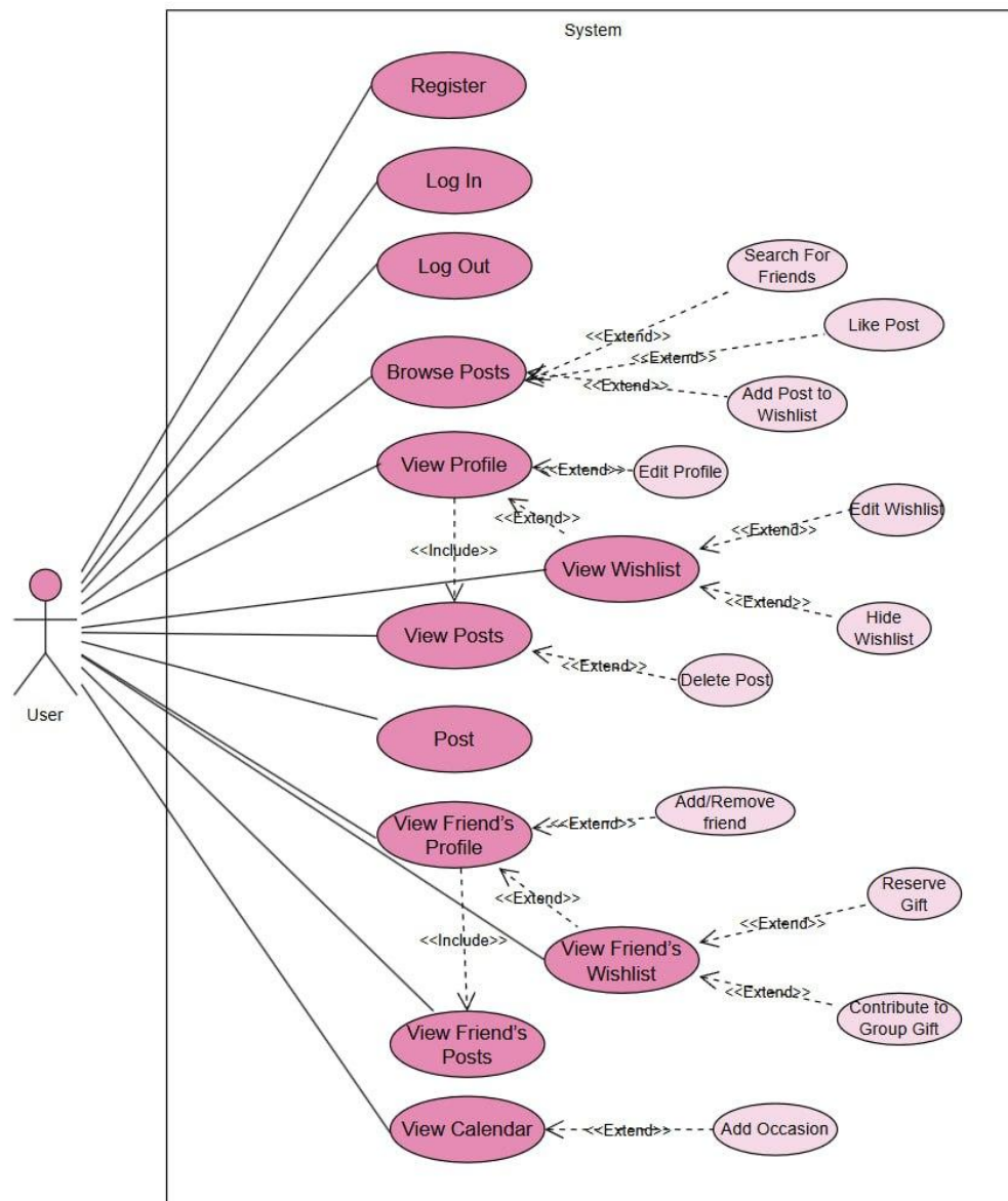
Figure 2: Use Case Diagram of WOD
