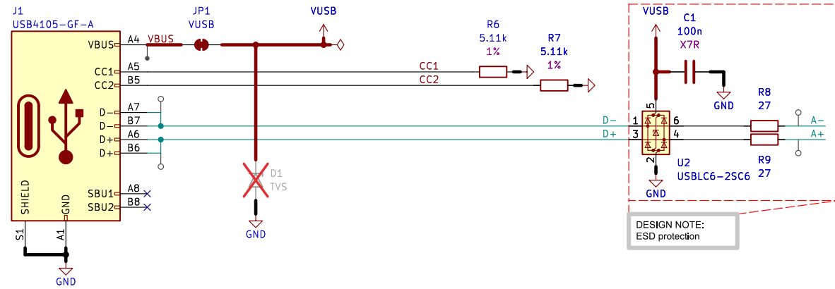
USB-C 2.0 INTERCONNECT
