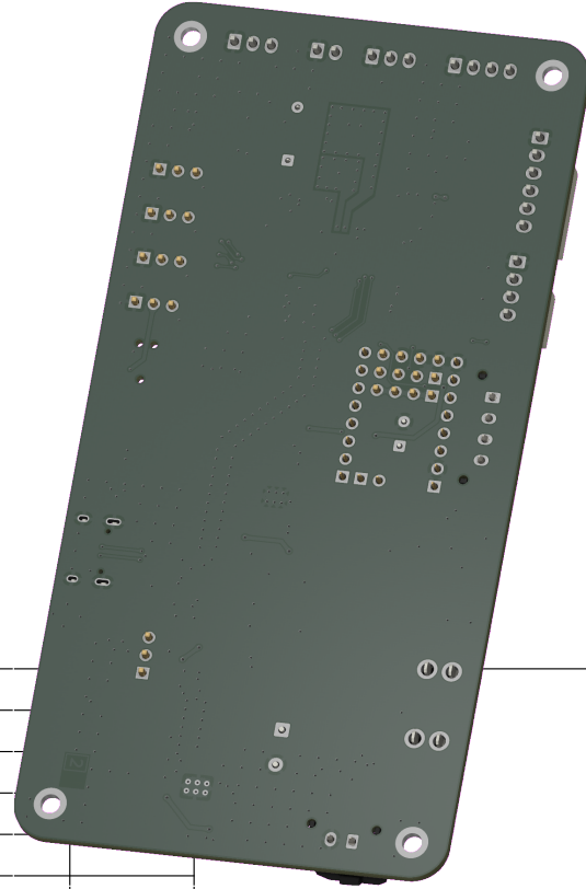
BOTTOM VIEW
