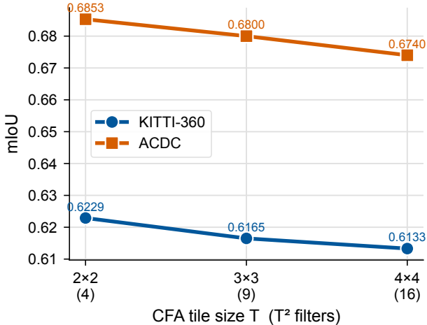
mIoU vs CFA Tile Size
