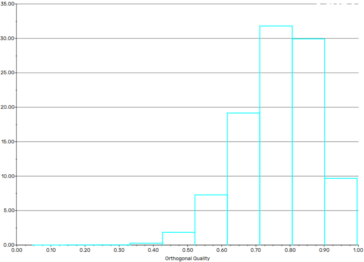
Histogram of Orthogonal Quality
