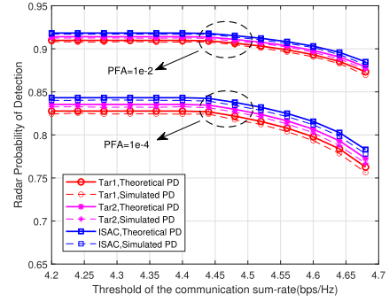
Fig. 7. Sensing P_D versus communication threshold in the comprehensiveness scheme.
