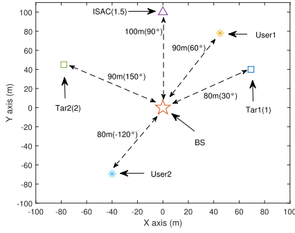
Fig. 9. Geometric distribution of the targets and users in the localization task.
