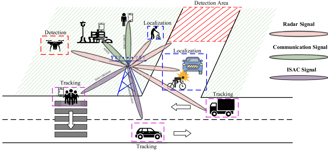
Fig. 1. Application scenarios of a single ISAC BS, providing communication and device-free sensing services simultaneously.
