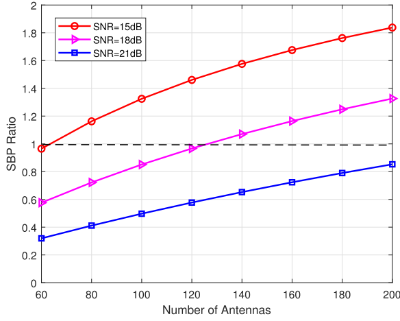
Fig. 5. Illustration of the trade-off between the bandwidth and spatial resources. The AoAs of three user are [-30^\circ, 0^\circ, 30^\circ] , where the reference user locates at \theta = 0^\circ . SNR is defined as 10\log(\kappa^2/\sigma_{\text{eff}}^2) , and B_q = 1/3B_{\text{total}} .
