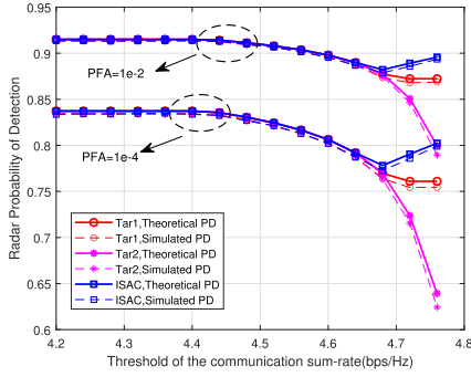
Fig. 6. Sensing P_D versus communication threshold in the fairness scheme.
