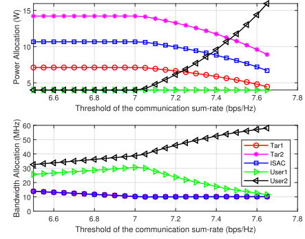
Fig. 11. Power and bandwidth allocation results.
