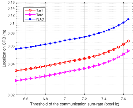
Fig. 10. Localization CRBs for sensing targets versus communication threshold.
