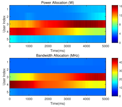
Fig. 13. RA results with the initial state \xi'_3 , \Gamma_c = 7.6 bps/Hz.
