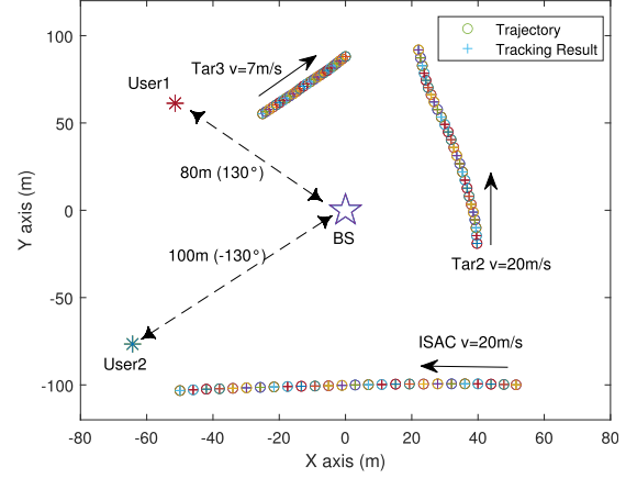
Fig. 15. Geometric distribution of the targets and users as well as the trajectory and tracking results for the moving targets, \Gamma_c = 7.6 bps/Hz.
