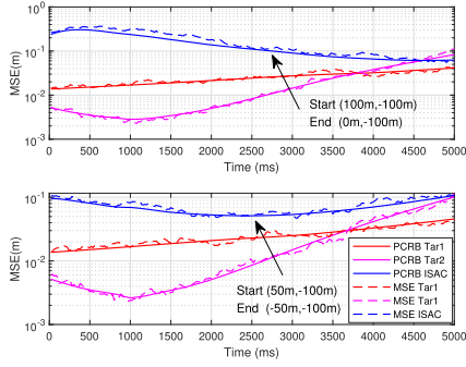
Fig. 12. Distance tracking performance PCRB for the moving targets with \Gamma_c = 7.6 bps/Hz.
