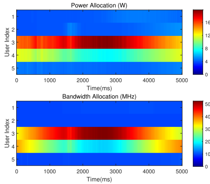
Fig. 14. RA results with the initial state \xi_3 , \Gamma_c = 7.6 bps/Hz.
