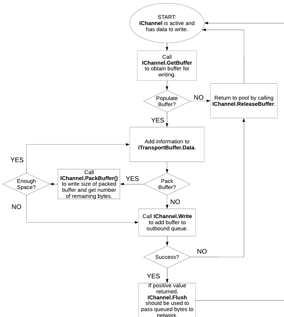
Figure 32. Enterprise Transport API Writing Flow Chart
