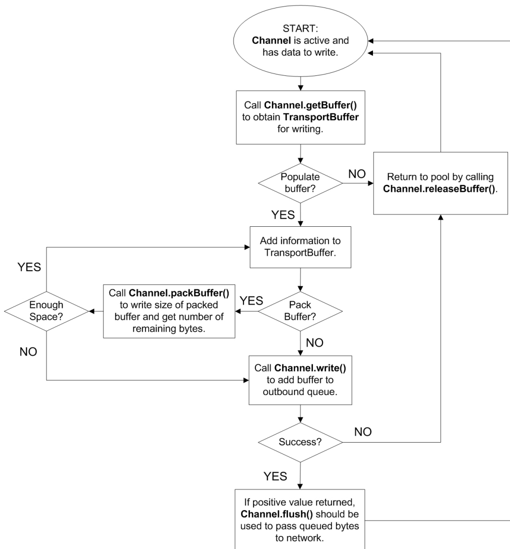
Figure 35. Enterprise Transport API Writing Flow Chart
