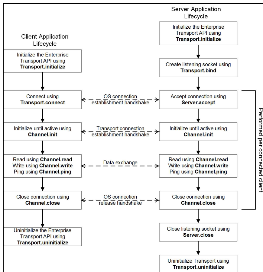
Figure 28. Transport Application Lifecycle
