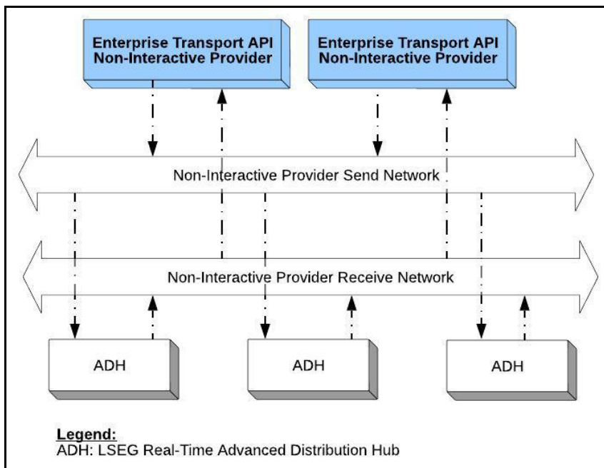
Figure 33. Multicast Connection Creation
