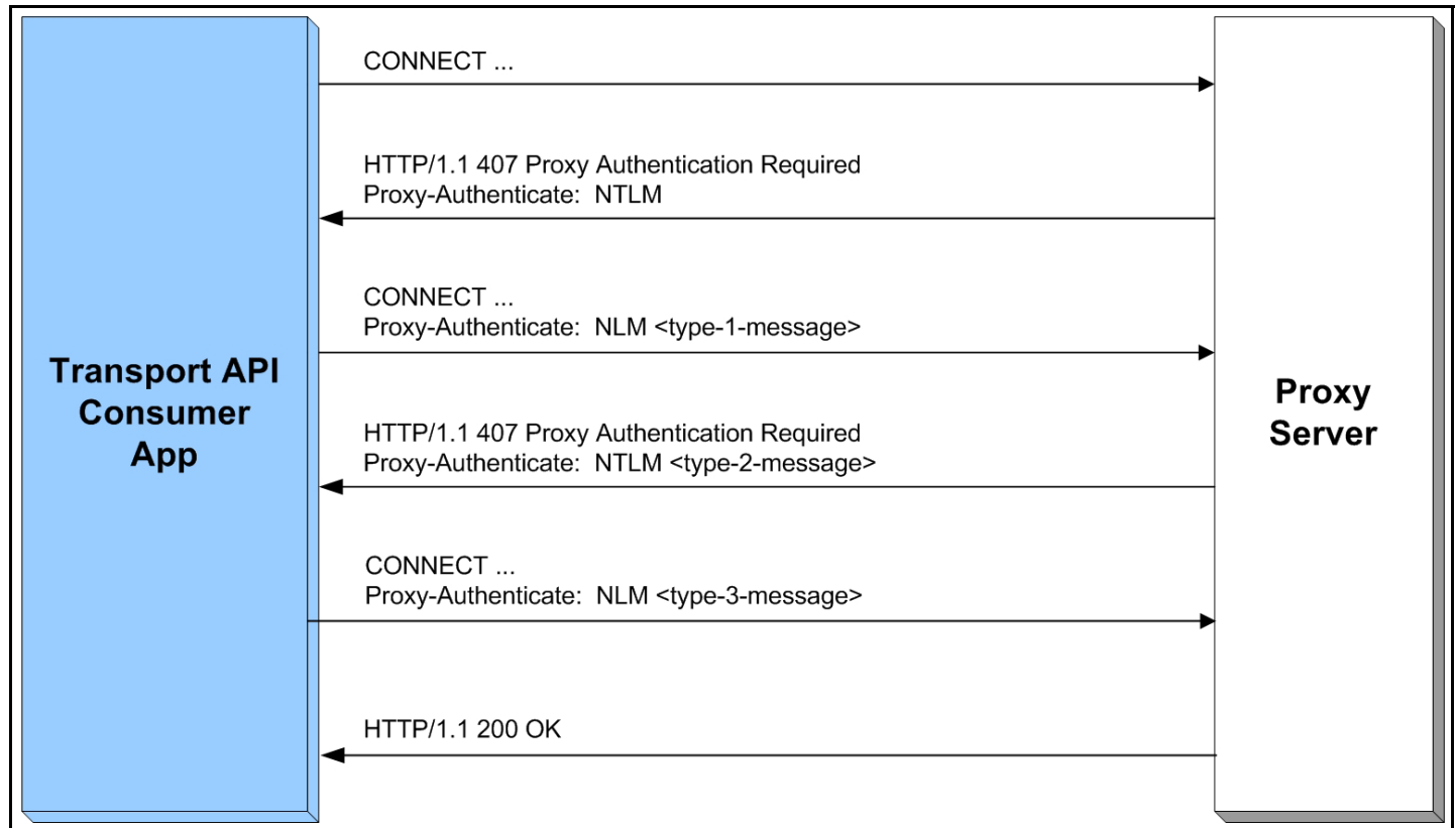
Figure 37. Enterprise Transport API Consumer Application authenticating with a Proxy Server using NTLM
