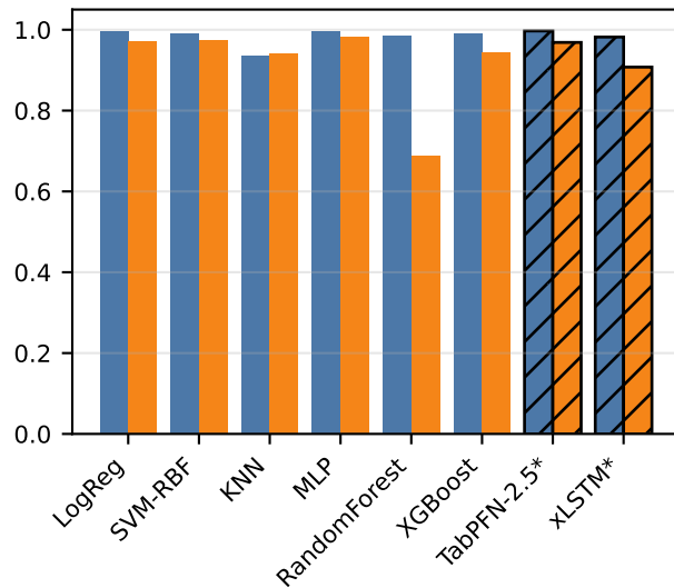
Severity (within-1)
