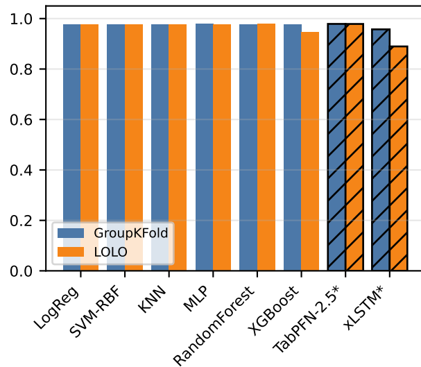
Detection (macro-F1)
