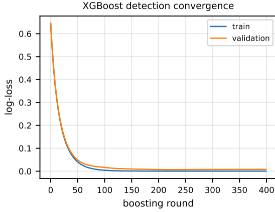
Fig. 12. Training behaviour. Left: XGBoost detection convergence (train/validation log-loss vs. boosting round). Right: 1-D CNN learning curves (training loss and validation macro-F1 vs. epoch), showing stable convergence without over-fitting.
