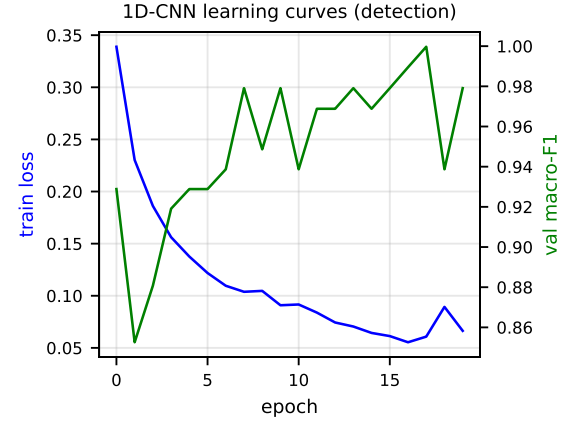
Fig. 12. Training behaviour. Left: XGBoost detection convergence (train/validation log-loss vs. boosting round). Right: 1-D CNN learning curves (training loss and validation macro-F1 vs. epoch), showing stable convergence without over-fitting.
