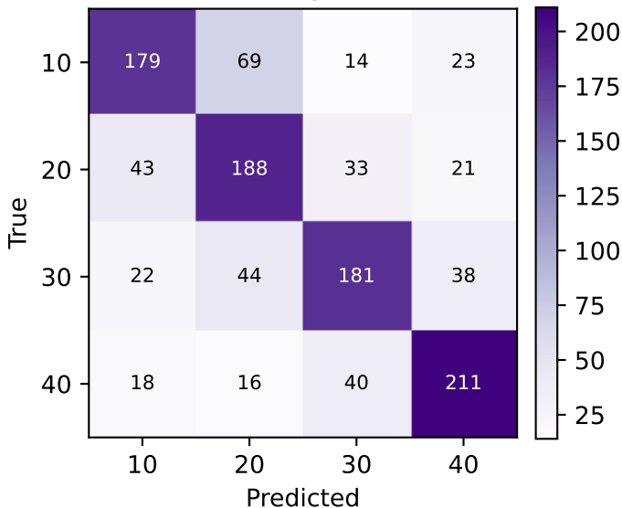
Hardware severity (XGBoost, GK)
