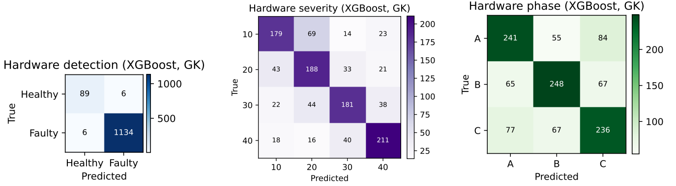
Fig. 12. Within-hardware confusion matrices on the real motor (XGBoost, GroupKFold out-of-fold): detection (left), four-level severity (middle), faulted phase (right). Detection is clean and severity errors are near-diagonal, but the phase matrix shows substantial off-diagonal confusion—the main simulation-to-reality gap.
