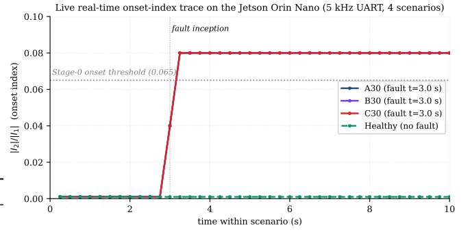
Fig. 15. Per-window onset index |I_2|/|I_1| over time for the four live-source scenarios on the Jetson Orin Nano. The healthy-only trace (green dashed) remains below 0.001 for the entire 10 s, never crossing the Stage-0 threshold (dotted horizontal line). Each faulted trace (A30/B30/C30, solid) jumps from \sim 0.001 to \sim 0.080 within one 250 ms window of the inception instant ( t=3.0 s, dotted vertical line), and the gated Stage 3 head then reports the correct faulted phase on each.
