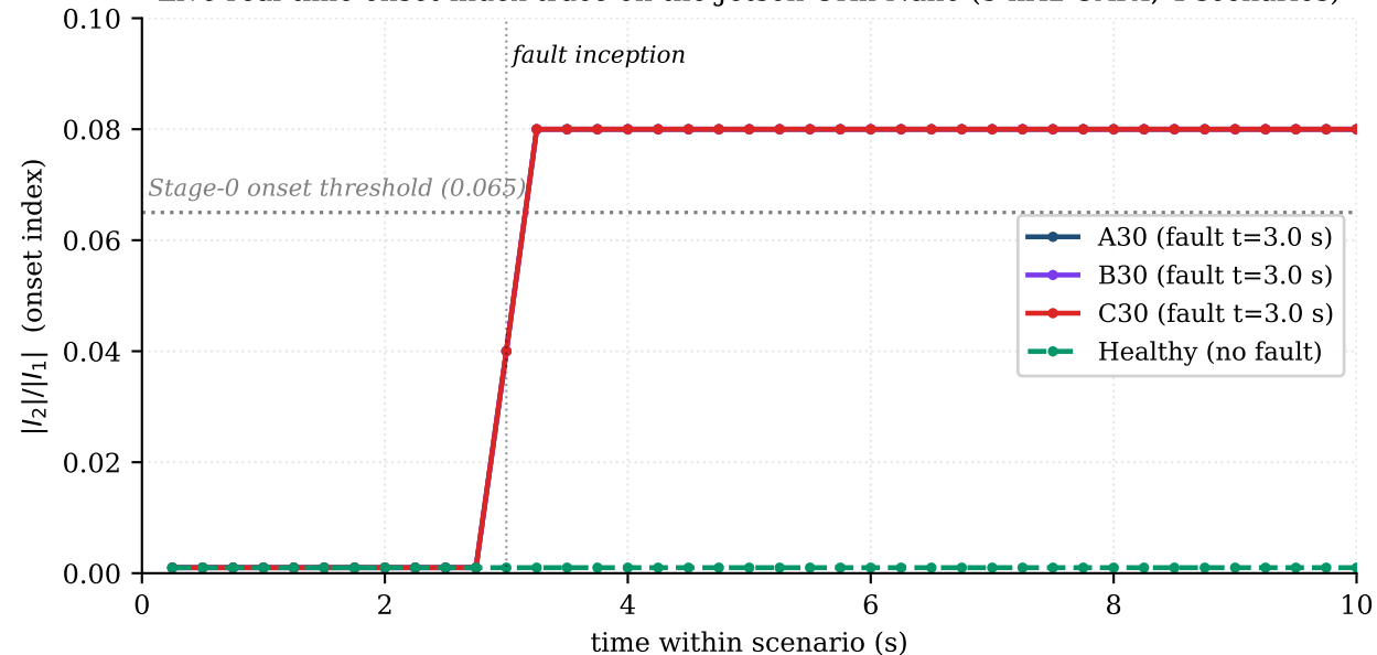
Live real-time onset-index trace on the Jetson Orin Nano (5 kHz UART, 4 scenarios)
