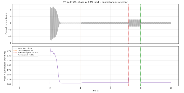
Fig. 2. Phase-A current (top) and per-cycle RMS envelope (bottom) of a faulted record, with motor start (2.0 s), load change (4.0 s), fault inception (7.2 s), and clearing (8.0 s). The fault interval supplies faulty windows; the pre-fault loaded region supplies matched-load healthy windows.
