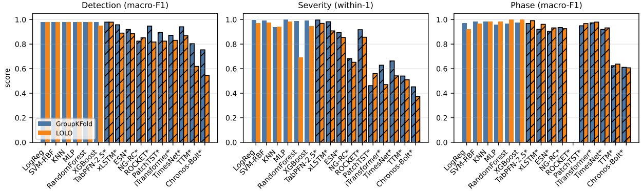
Fig. 8. 14-model benchmark across the three diagnostic tasks under both protocols (GroupKFold vs. LOLO). Hatched bars denote models added in this work (TabPFN-2.5, xLSTM, ESN, NG-RC, ROCKET, PatchTST, iTransformer, TimesNet, TTM, Chronos-Bolt). Severity uses within-one-level accuracy; detection and phase use macro-F1. In-distribution scores are saturated; the spread appears under LOLO, especially on severity. The tabular feature classifiers own detection and severity LOLO; the modern attention models (iTransformer, PatchTST) close the phase-ID gap without engineered features; the two time-series foundation models trail substantially under LOLO.
