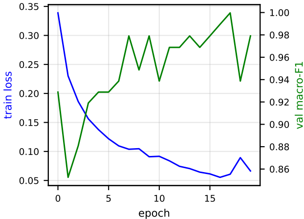
1D-CNN learning curves (detection)
