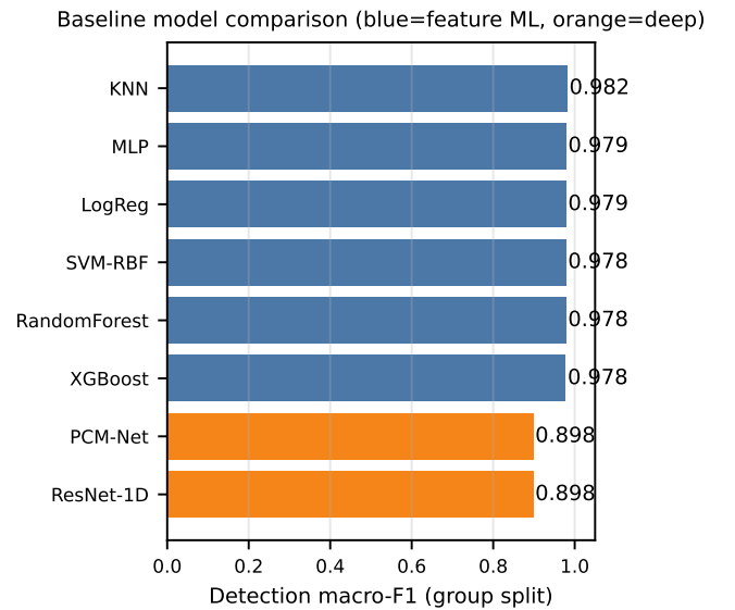
Fig. 8. Baseline model comparison on detection (five-fold mean macro-F1). Feature-based ML (blue) clusters high; raw-signal deep models (orange) trade in-distribution detection for their cross-load severity edge.
