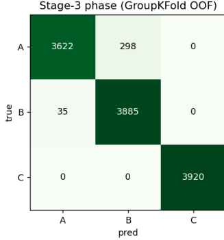
Fig. 2. Faulted-phase confusion (group k -fold, out-of-fold). Phase C is perfect; only minor A \leftrightarrow B confusion remains. Cross-load (LOLO) phase accuracy is 0.997.
