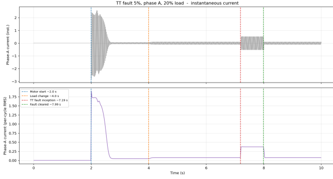
Fig. 1. Phase-A current (top) and per-cycle RMS envelope (bottom) of a faulted record, with motor start (2.0 s), load change (4.0 s), fault inception (7.2 s), and clearing (8.0 s). The fault interval supplies faulty windows; the pre-fault loaded region supplies matched-load healthy windows.
