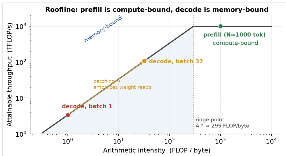
Figure 2. The H100 roofline. Decode at batch 1 ( \text{AI} \approx 1 ) is far down the memory-bound slope — its speed is set by HBM bandwidth, not FLOPs. Prefill ( \text{AI} \approx 1000 ) is past the ridge in the compute-bound flat. Batching decode walks the operating point right along the slope (§4.3).
