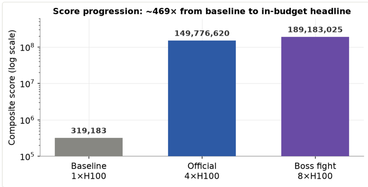
Figure 7. Score progression (log scale) from the unoptimized baseline (319K) to the in-budget headline (150M) and the scaled 8-GPU tier (189M) — a \sim 469\times lift end-to-end, \sim 54\times over the public reference baseline at the in-budget result.
