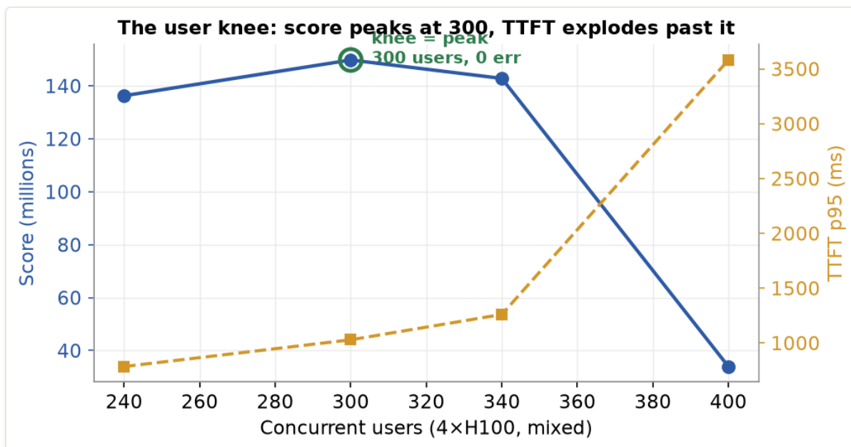
Figure 5. The user knee on 4xH100. Score (blue) peaks at 300 users; TTFT p95 (amber) stays near 1 s through the knee, then explodes 3.5x to 3.6 s by 400 users as the prefill queue saturates (Little's law, §4.5) — dragging the composite down even though more users are offered.
