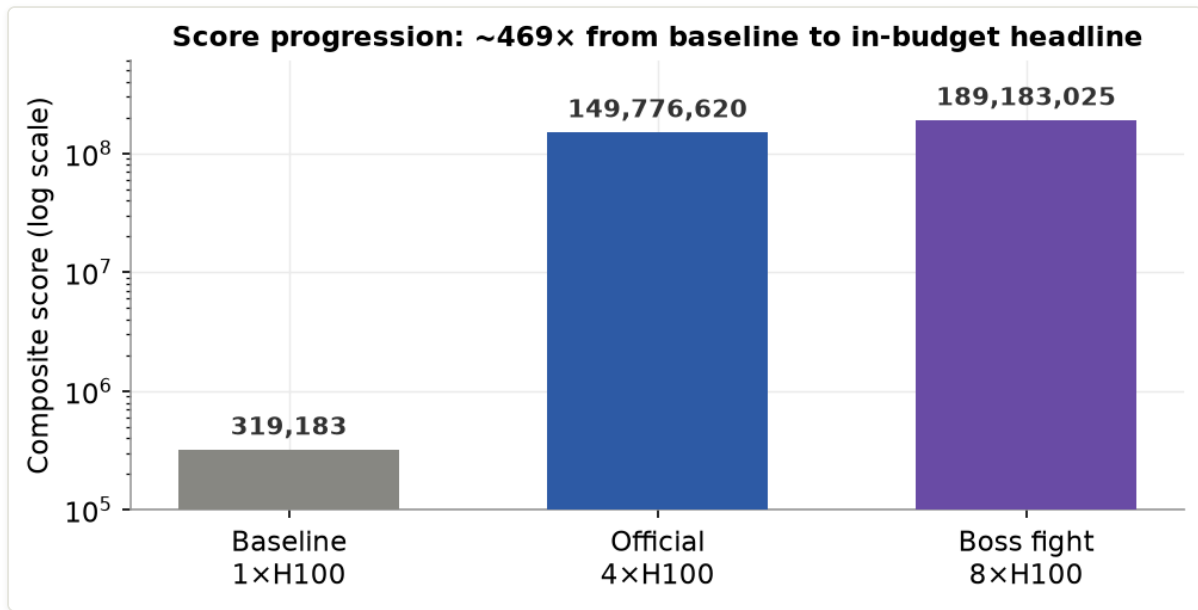
Figure 7. Score progression (log scale) from the unoptimized baseline (319K) to the in-budget headline (150M) and the optional boss fight (189M) — a ~469× lift end-to-end, ~54× over the spec's mixed reference at the in-budget result.
