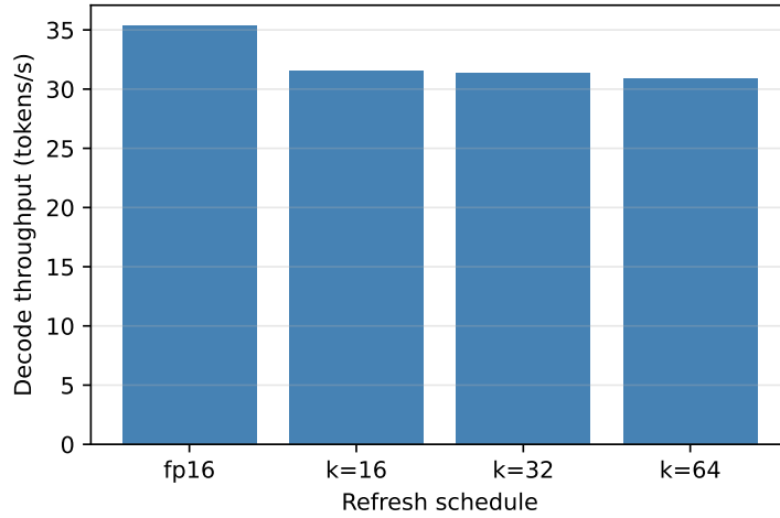
Figure 6: Measured decode throughput for the 4-bit refresh schedules versus the fp16 baseline (single GPU). Refresh costs a 1.12–1.14x slowdown largely independent of k .
