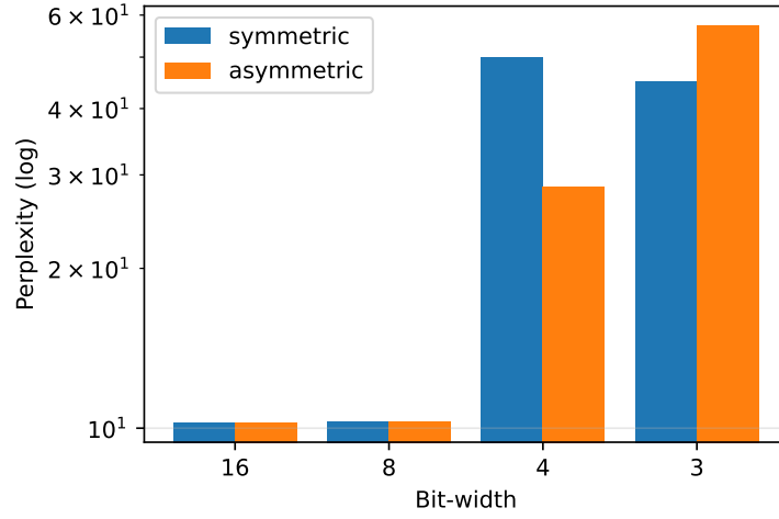
Figure 5: Symmetric vs. asymmetric state quantization (perplexity, log scale, 1.3b). Asymmetric rounding nearly halves the 4-bit penalty but does not help at 3-bit.
