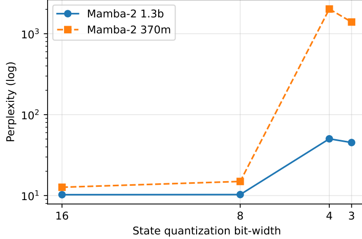
Figure 2: Perplexity versus state quantization bit-width (log scale). 8-bit tracks fp16 closely on the 1.3b model; 4-bit and 3-bit fall off a cliff. The 370m model leaves the lossless plateau even at 8-bit.
