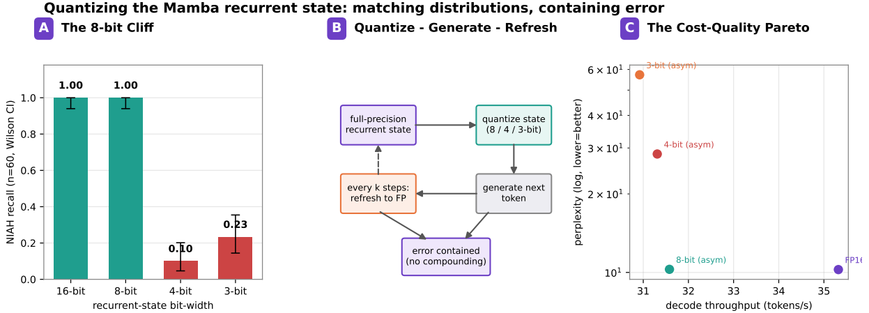
Figure 1: Overview. (A) NIAH recall by recurrent-state bit-width ( n=60 , Wilson 95% CIs): quantization is lossless to 8-bit but collapses sharply at 4-bit and below. (B) The post-training pipeline: quantize the recurrent state, generate, and optionally refresh to full precision every k steps to contain error. (C) The measured cost-quality Pareto across bit-widths (asymmetric quantization).
