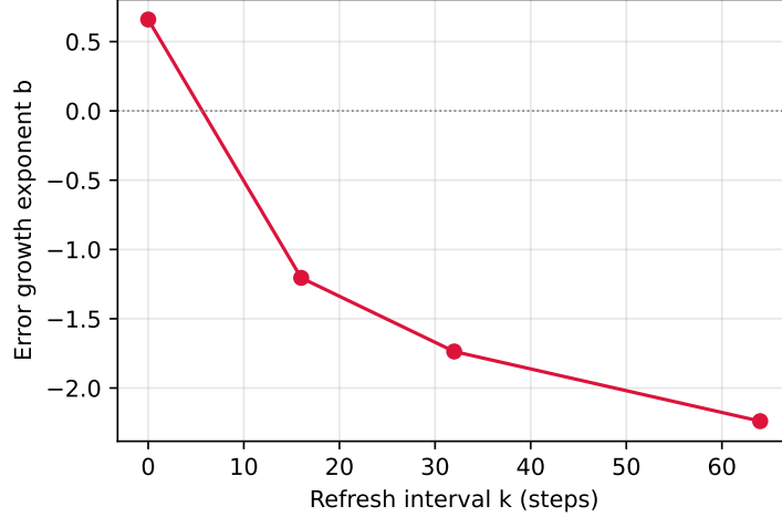
Figure 3: Error-growth exponent b versus refresh interval k under 4-bit quantization. b crosses from positive (compounding) to negative (contained) as refreshes become more frequent.
