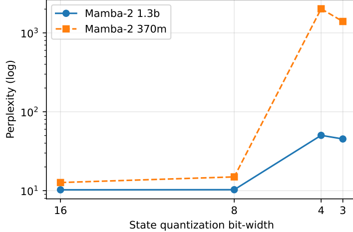
Figure 1: Perplexity versus state quantization bit-width (log scale). 8-bit tracks fp16 closely on the 1.3b model; 4-bit and 3-bit fall off a cliff. The 370m model leaves the lossless plateau even at 8-bit.
