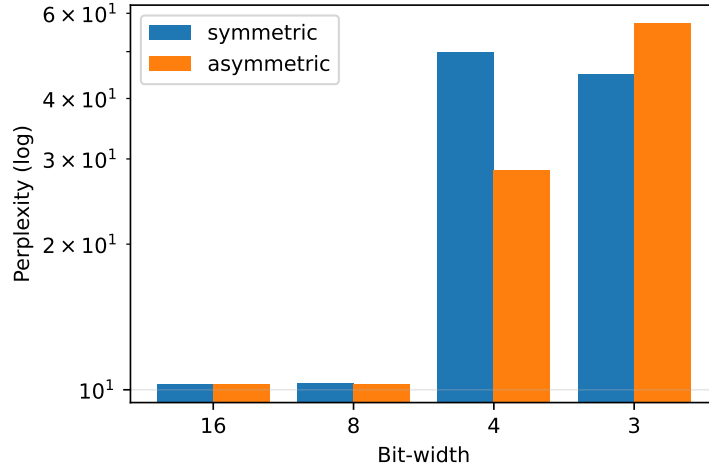
Figure 4: Symmetric vs. asymmetric state quantization (perplexity, log scale, 1.3b). Asymmetric rounding nearly halves the 4-bit penalty but does not help at 3-bit.
