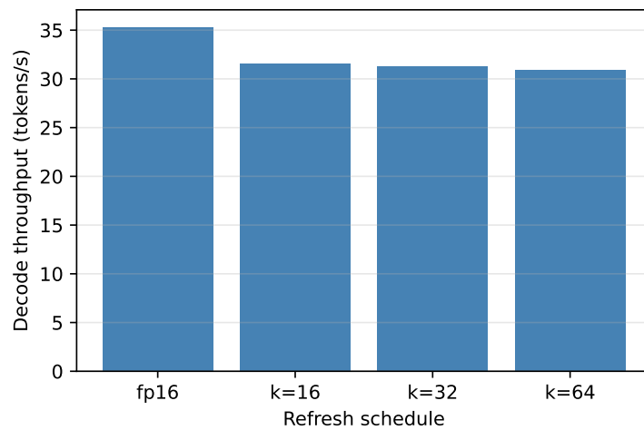
Figure 5: Measured decode throughput for the 4-bit refresh schedules versus the fp16 baseline (single GPU). Refresh costs a 1.12–1.14x slowdown largely independent of k .
