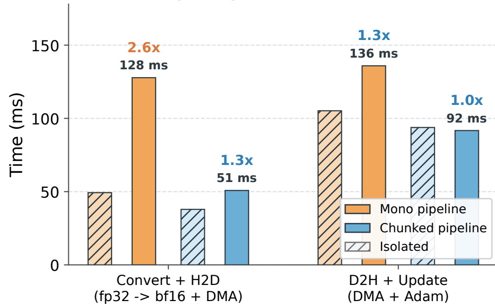
Pipeline Component Breakdown (single layer, 64 MiB chunks)
