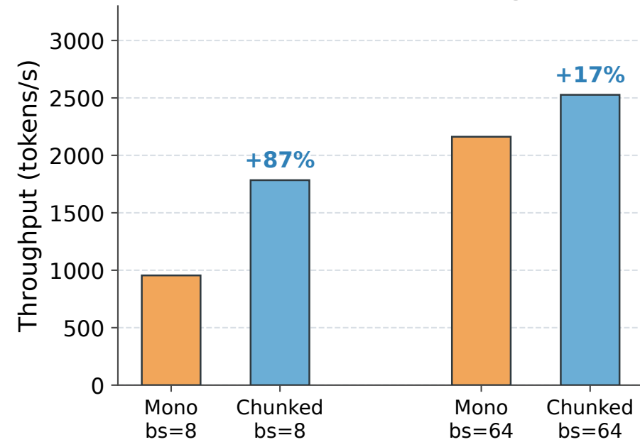
Full Model (Qwen3-8B, RTX 4090) end-to-end training
