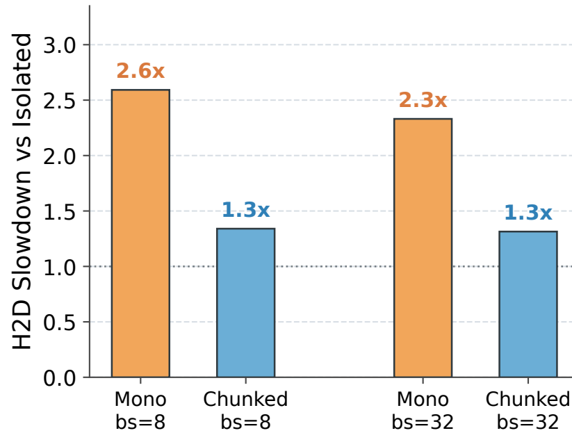
H2D PCIe Interference (lower = better)
