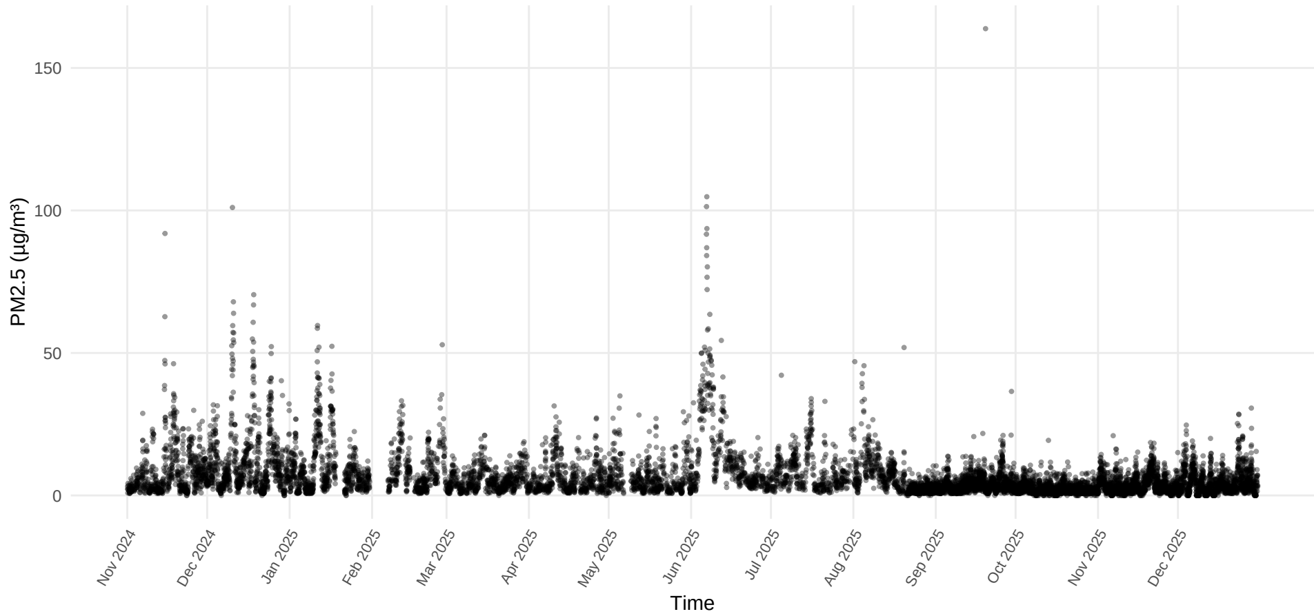
PM2.5 Time Series – Device 15 – Coit Road and East 131st Street
