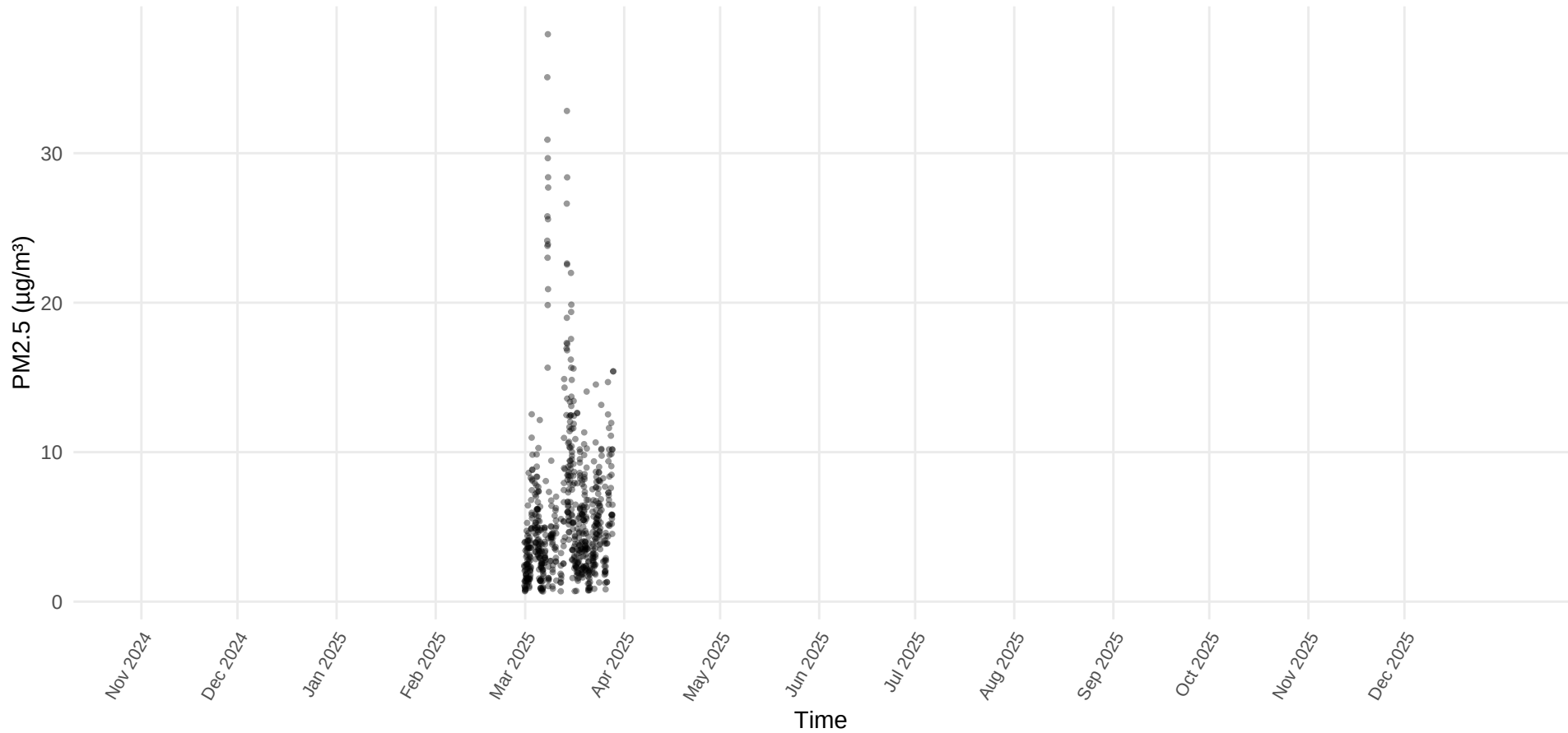
PM2.5 Time Series – Site 17.1 (Device 17 – Michael Zone Recreation Center )
