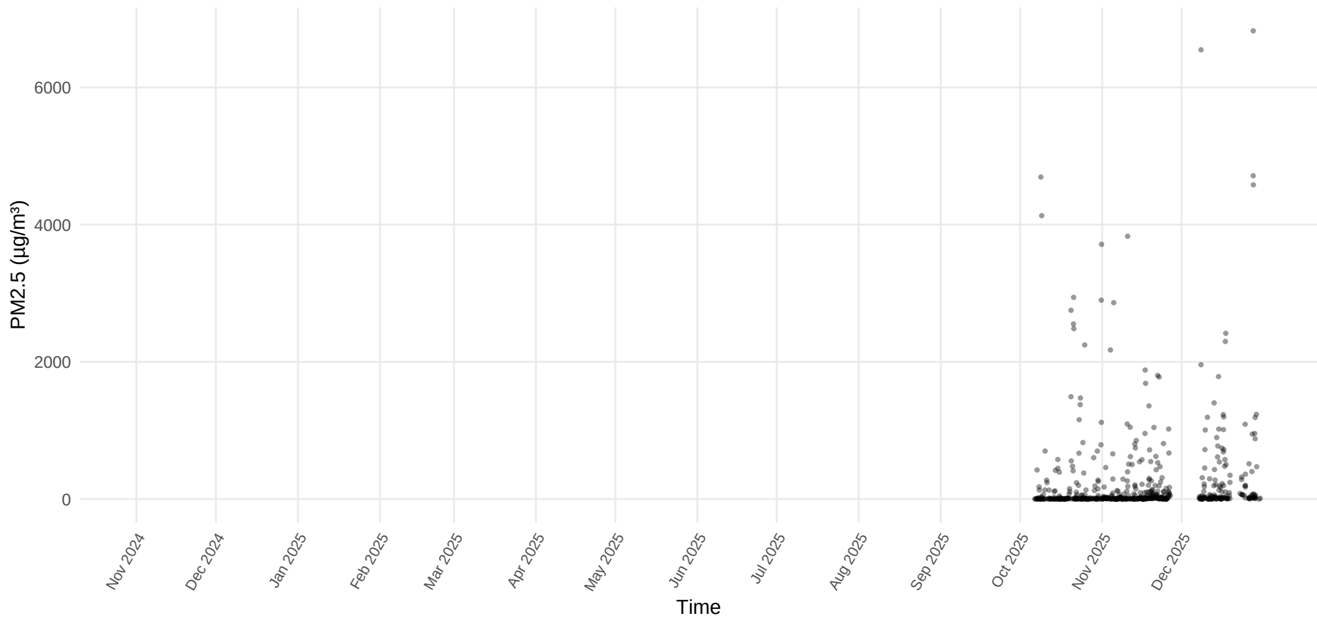
PM2.5 Time Series – Site 18.2 (Device 18 – East 166th St. and St. Clair Ave. )
