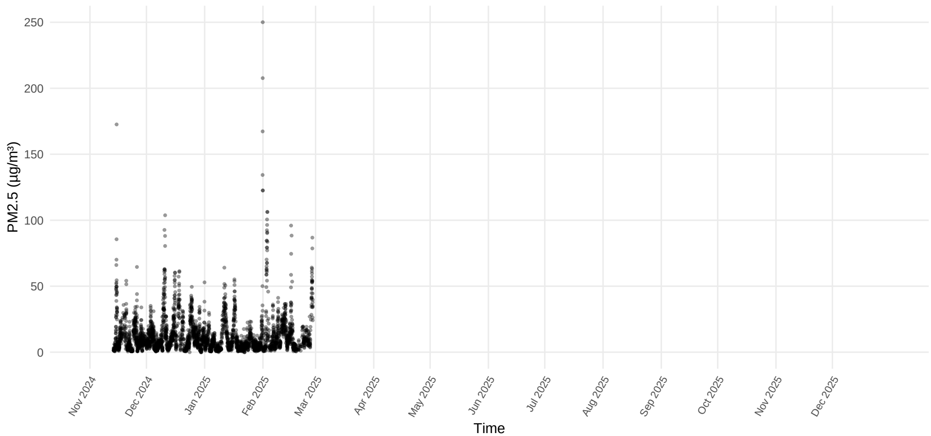
PM2.5 Time Series – Site 30.1 (Device 30 – Michael Zone Recreation Center )
