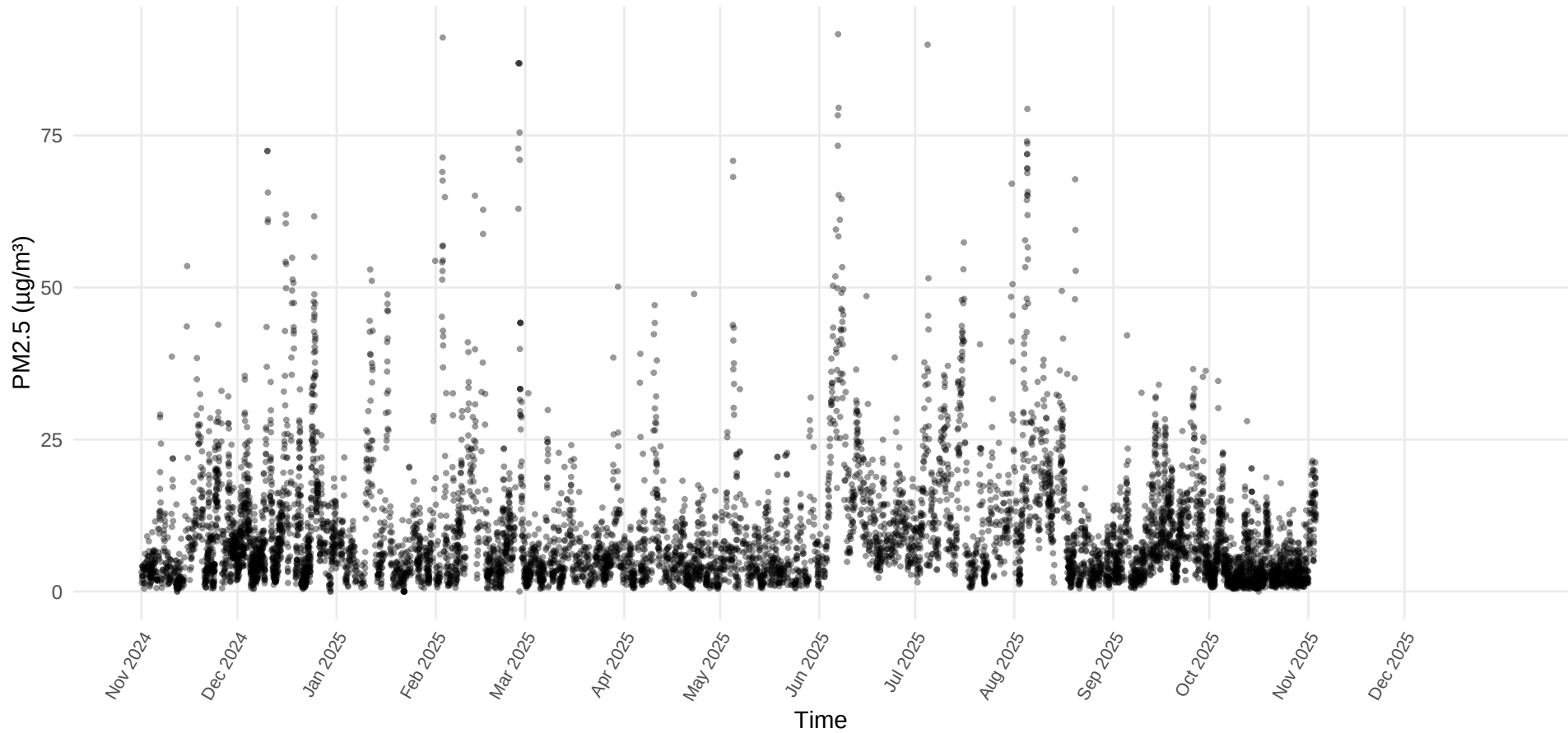
PM2.5 Time Series – Site 8.1 (Device 8 – East 56th Street and Ferro Avenue )
