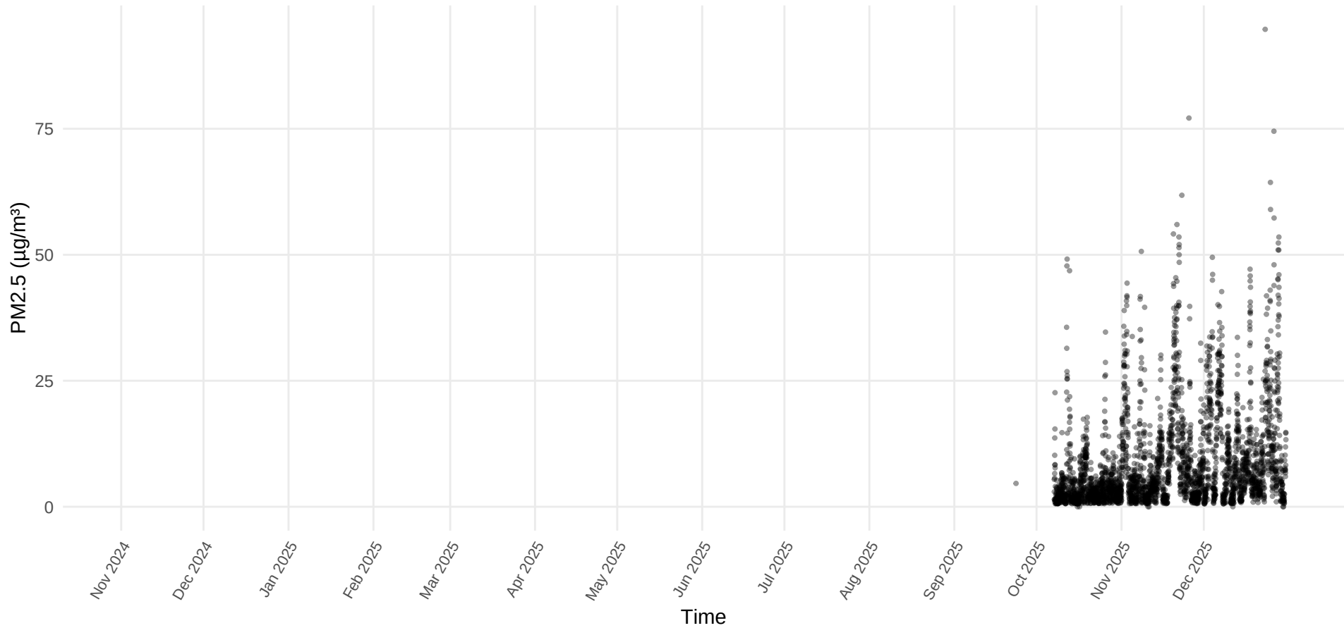
PM2.5 Time Series – Device 16 – In office (testing)
