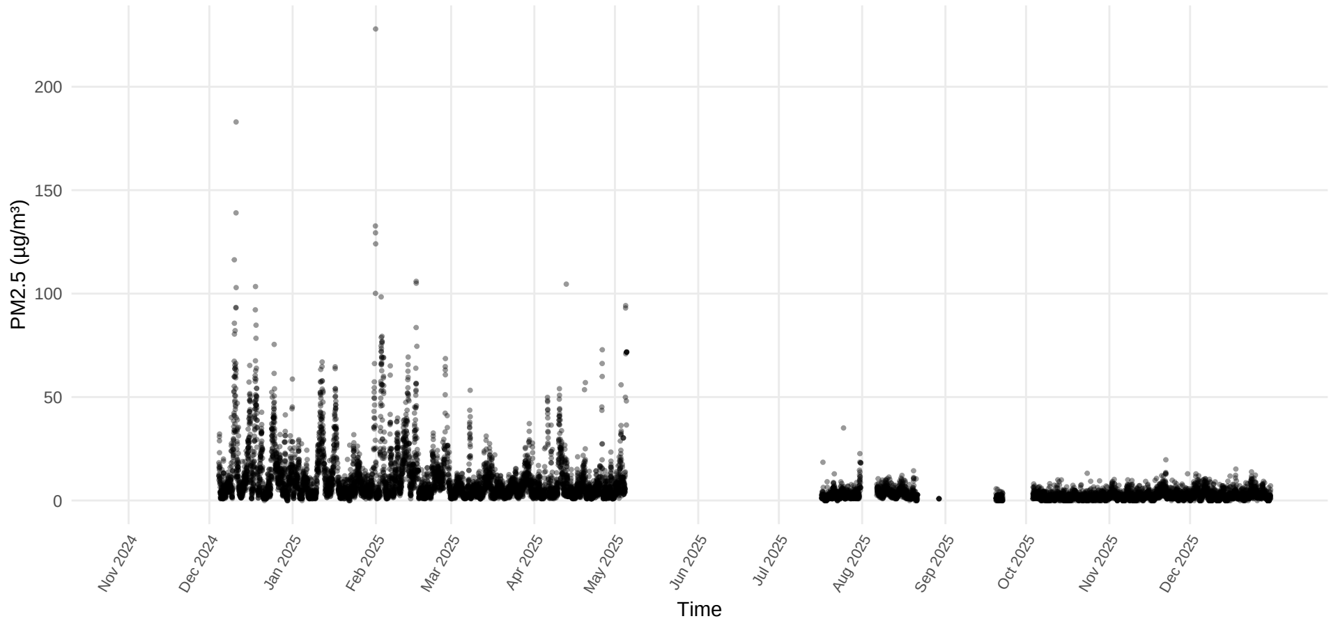
PM2.5 Time Series – Device 28 – Metro Health Hospital
