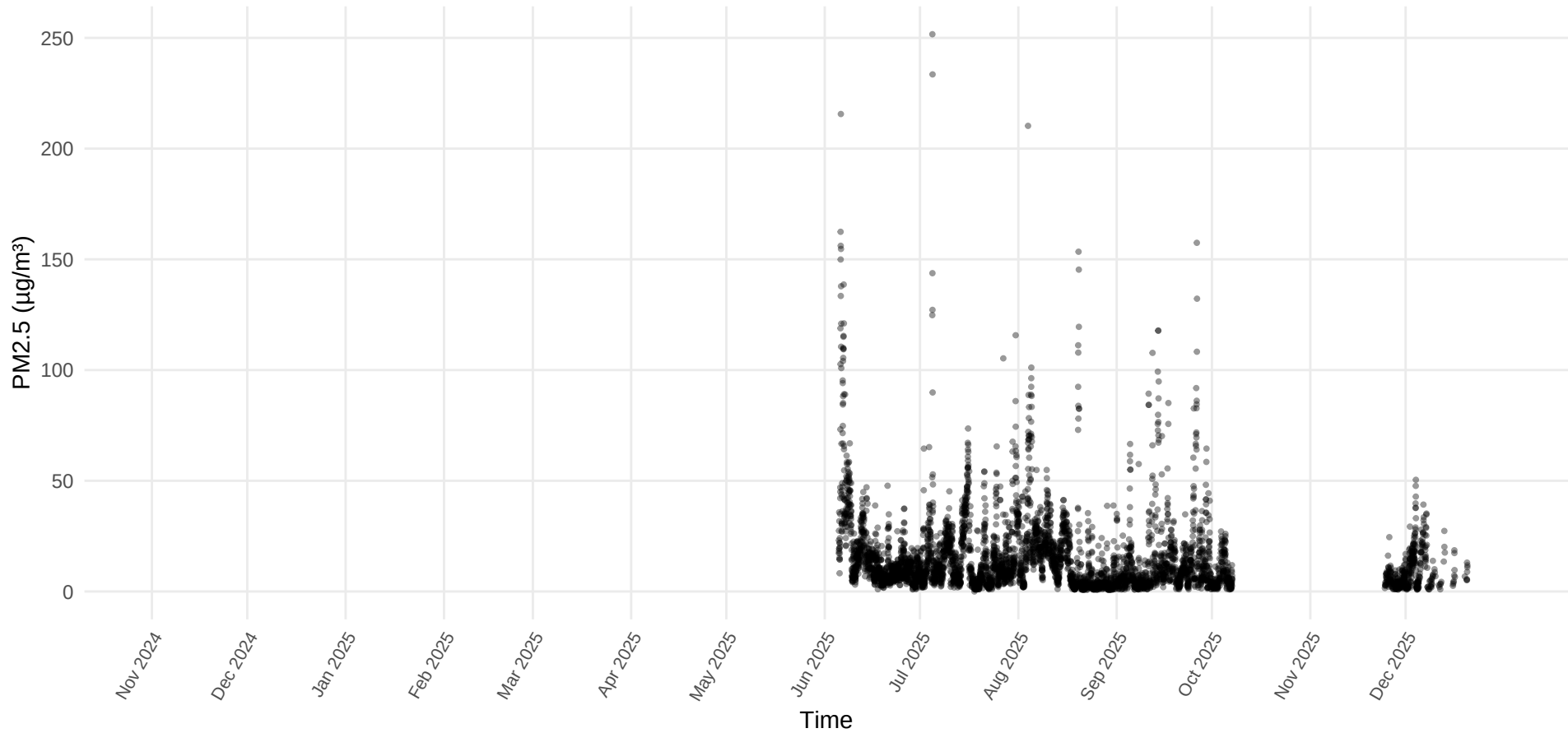
PM2.5 Time Series – Device 34 – Clark Recreation Center
