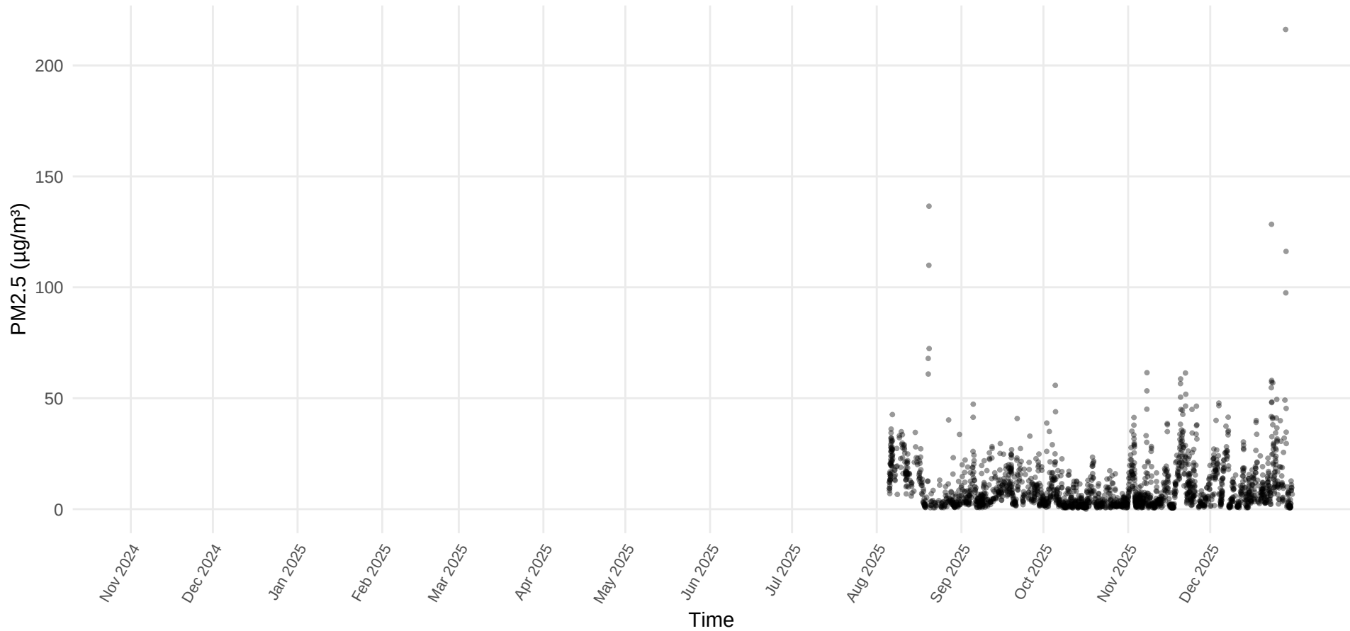
PM2.5 Time Series – Device 4 – St. Theodosius Monitoring Site Collocated Sensor
