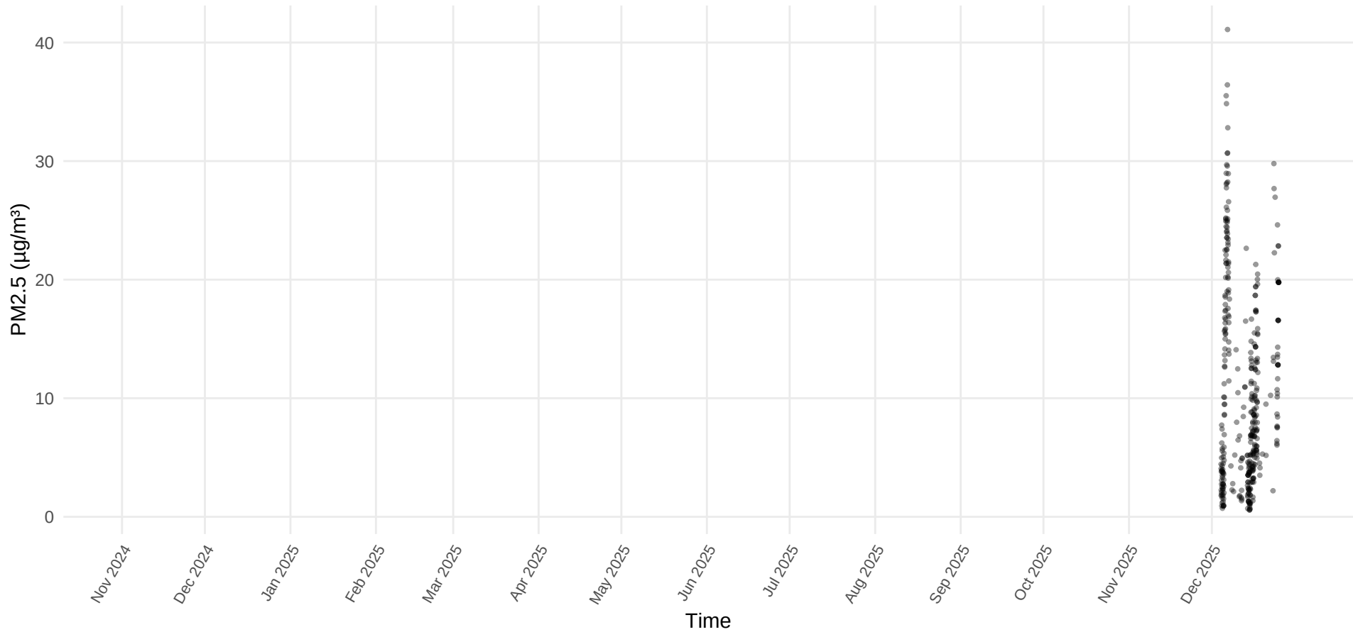
PM2.5 Time Series – Site 11.3 (Device 11 – Cleveland Fire #7 )
